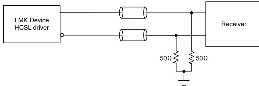
Figure 7-29. DC-Coupled HCSL Output Termination
