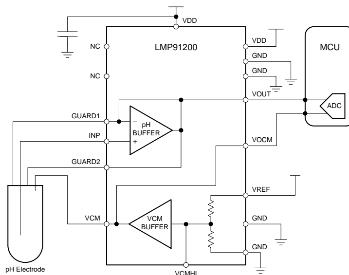
Figure 34. Typical Application
