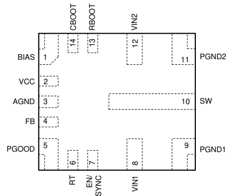
Figure 5-1. RJR Package 14-Pin VQFN-HR Top View
