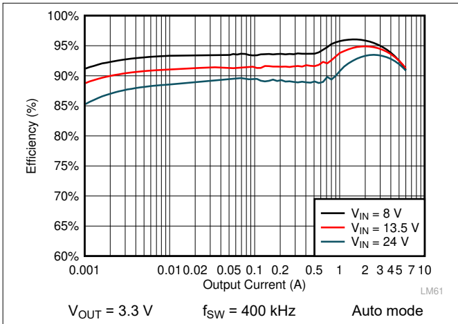
Figure 8-5. LMQ61460 Efficiency
