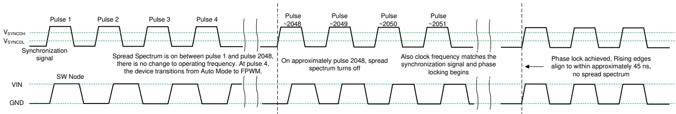
Figure 7-5. Synchronization Process
