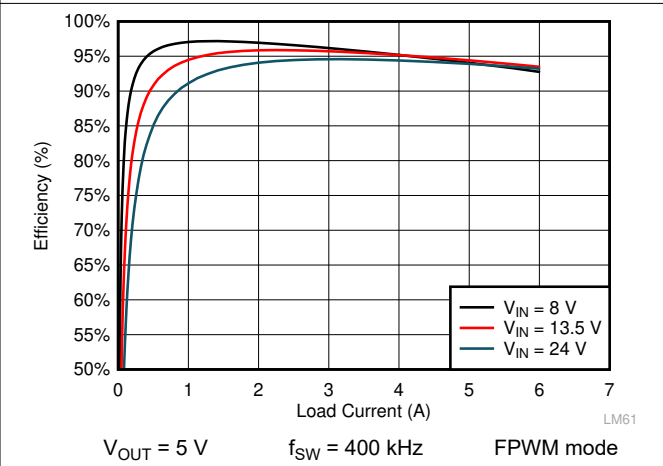
Figure 8-10. LMQ61460 Efficiency
