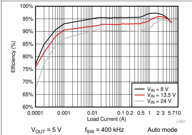
Figure 8-9. LMQ61460 Efficiency
