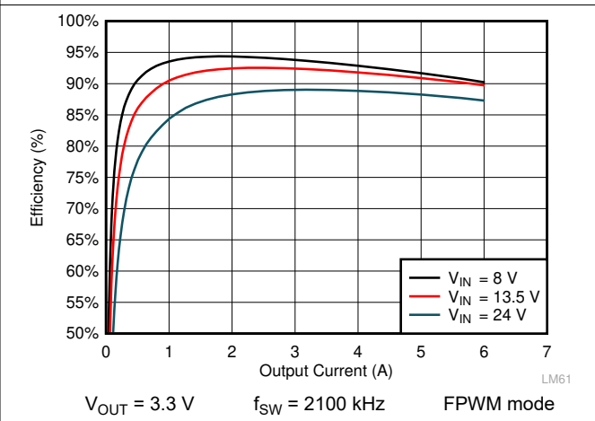
Figure 8-8. LMQ61460 Efficiency
