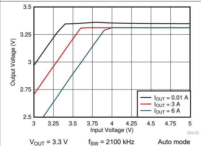
Figure 9-22. LMQ61460 Dropout Curve
