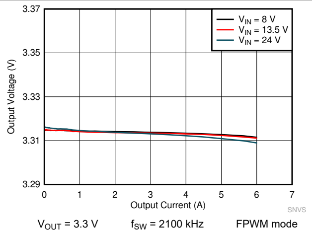
Figure 8-16. LMQ61460 Load and Line Regulation
