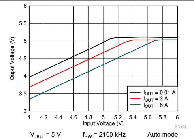
Figure 8-24. LMQ61460 Dropout Curve
