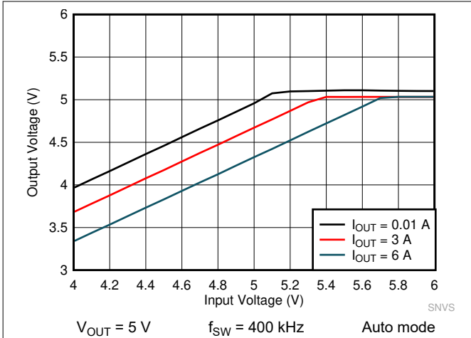
Figure 8-23. LMQ61460 Dropout Curve
