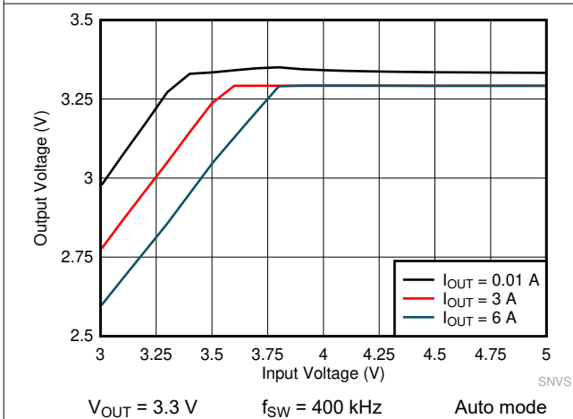
Figure 9-21. LMQ61460 Dropout Curve
