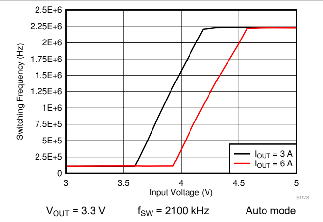
Figure 8-26. LMQ61460 Frequency Dropout Curve
