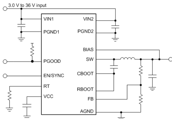
Simplified Schematic
