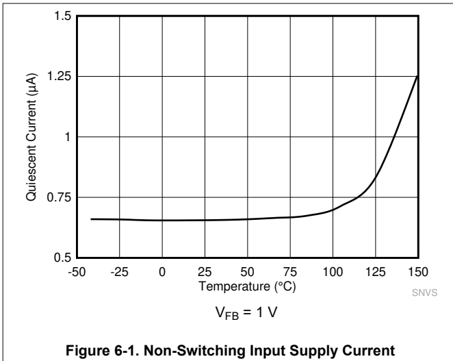
Figure 6-1. Non-Switching Input Supply Current
