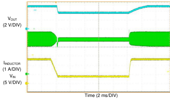
Figure 8-35. LMQ61460 Short-Circuit Recovery
