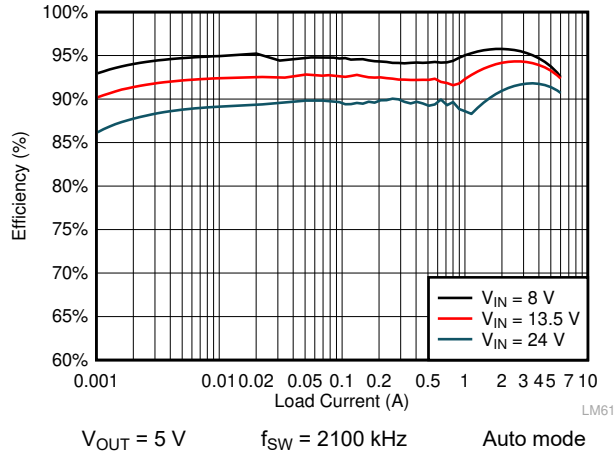
Figure 8-11. LMQ61460 Efficiency
