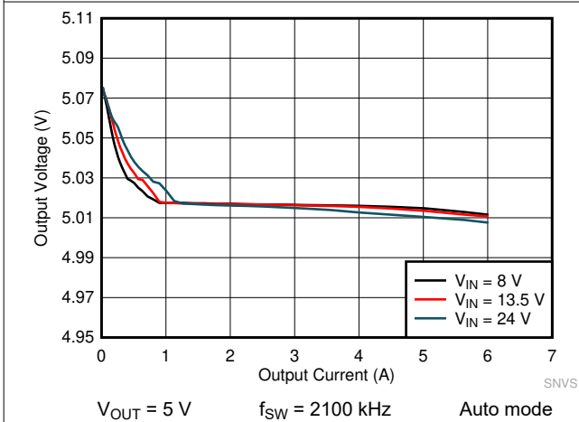
Figure 9-19. LMQ61460 Load and Line Regulation
