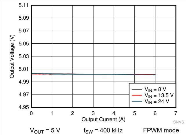
Figure 9-18. LMQ61460 Load and Line Regulation
