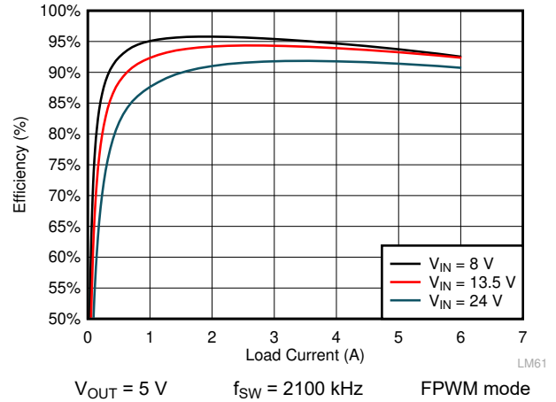
Figure 8-12. LMQ61460 Efficiency
