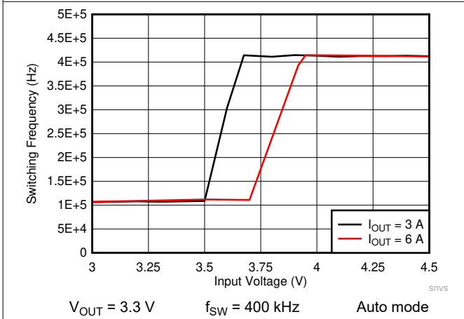
Figure 8-25. LMQ61460 Frequency Dropout Curve
