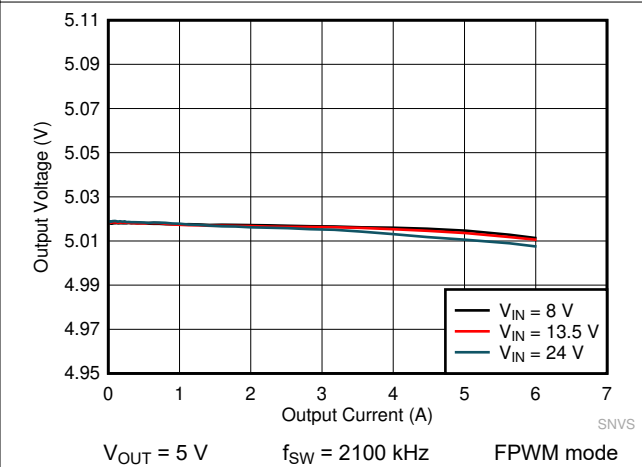
Figure 9-20. LMQ61460 Load and Line Regulation
