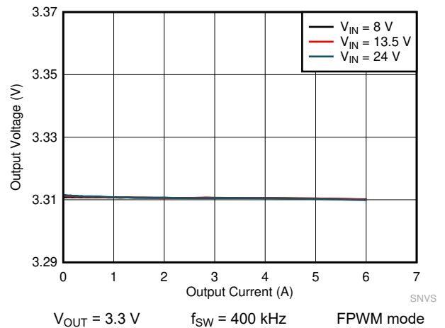
Figure 8-14. LMQ61460 Load and Line Regulation
