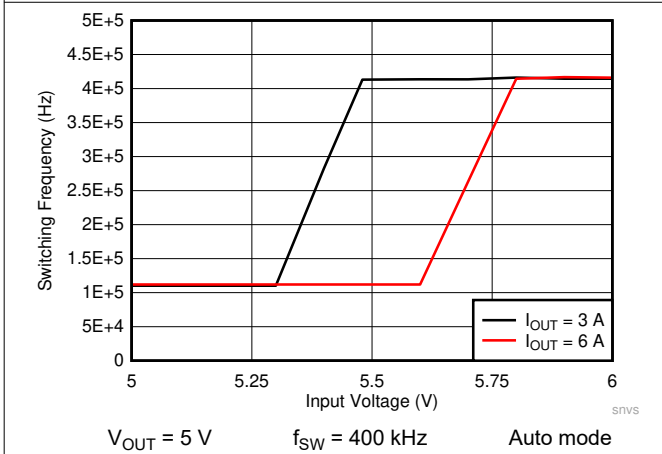
Figure 8-27. LMQ61460 Frequency Dropout Curve
