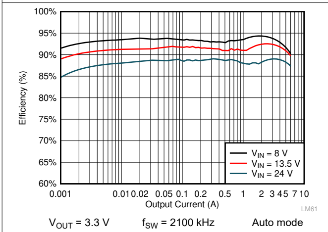
Figure 8-7. LMQ61460 Efficiency
