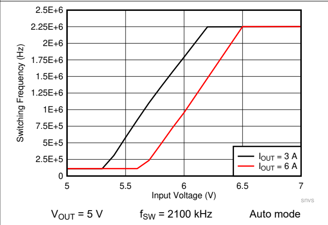
Figure 8-28. LMQ61460 Frequency Dropout Curve
