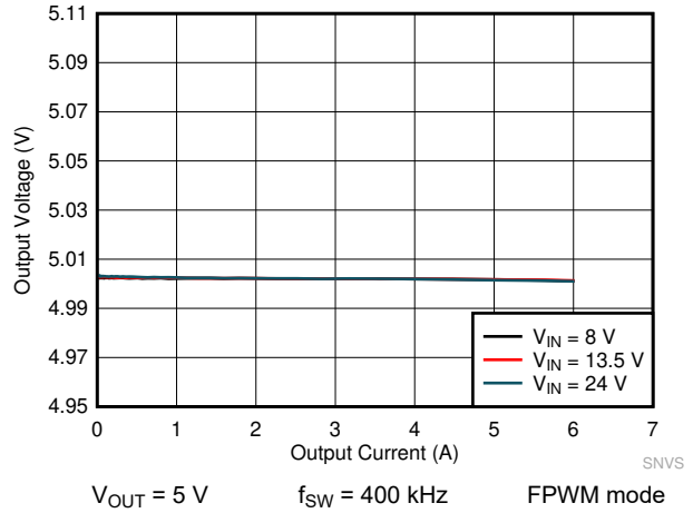
Figure 8-18. LMQ61460 Load and Line Regulation
