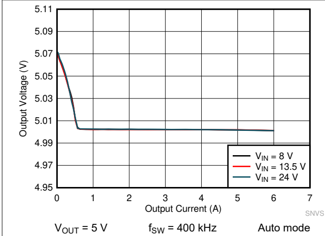
Figure 9-17. LMQ61460 Load and Line Regulation
