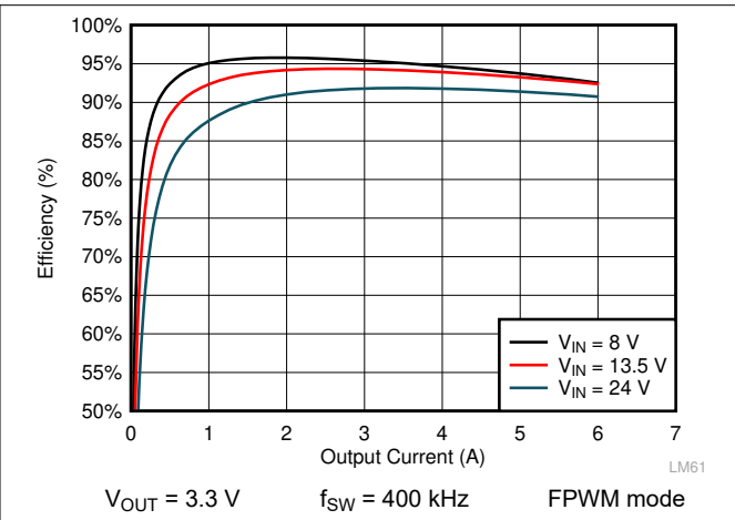
Figure 8-6. LMQ61460 Efficiency
