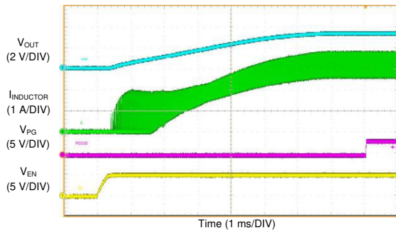
Figure 8-31. LMQ61460 Start-Up With 50-mA Load
