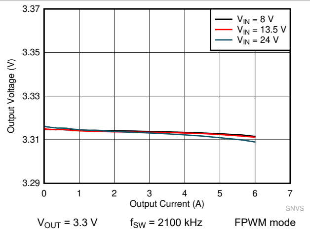
Figure 9-16. LMQ61460 Load and Line Regulation
