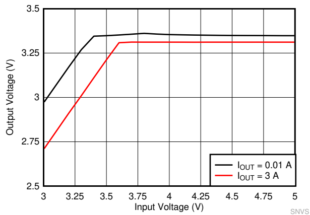
Figure 9-11. LMQ62440-Q1 Load and Line Regulation
