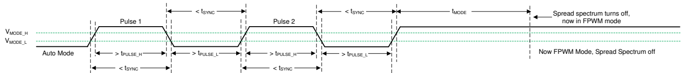
Figure 8-9. Spread Spectrum Disabled in Transition from Auto Mode to FPWM Mode
