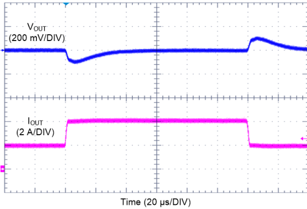
Figure 9-23. LMQ62440-Q1 Load Transient
