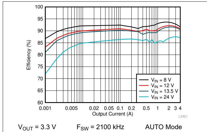
Figure 9-5. LMQ62440-Q1 Efficiency
