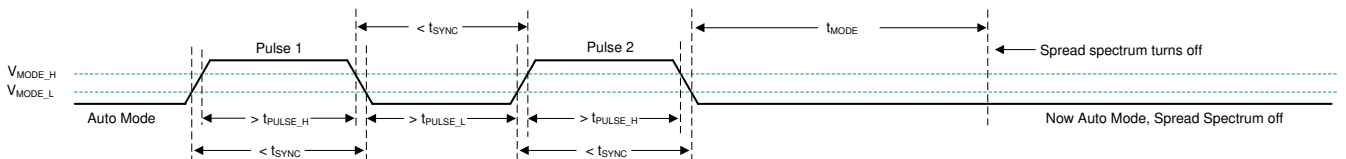
Figure 8-7. Spread Spectrum Disabled in Auto Mode
