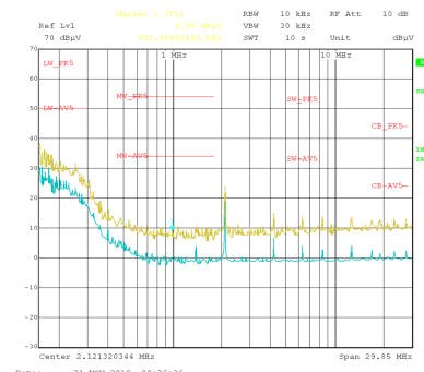
Figure 9-32. Radiated EMI Log Horizontal versus CISPR25 Limits
