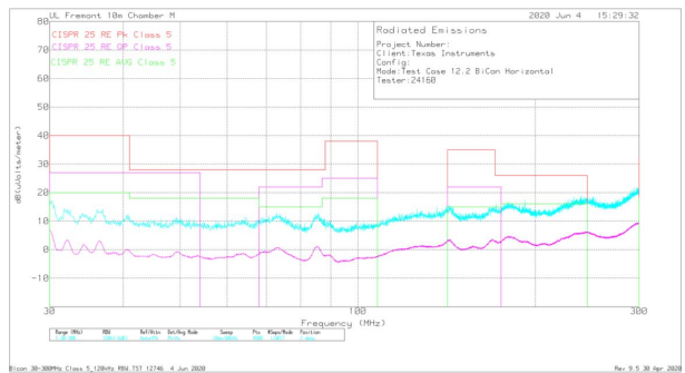
Figure 9-36. Radiated EMI Red versus CISPR25 Limits
