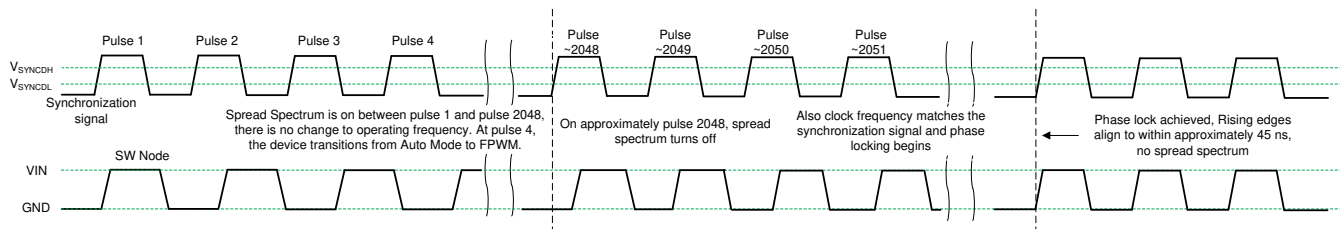
Figure 8-12. Synchronization Process
