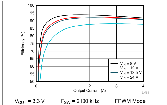
Figure 9-6. LMQ62440-Q1 Efficiency
