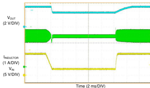
Figure 8-16. Recovery From Dropout
