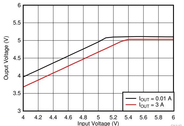
Figure 9-12. LMQ62440-Q1 Load and Line Regulation
