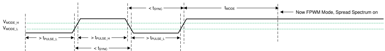
Figure 8-11. Transition from SYNC Mode to FPWM Mode
