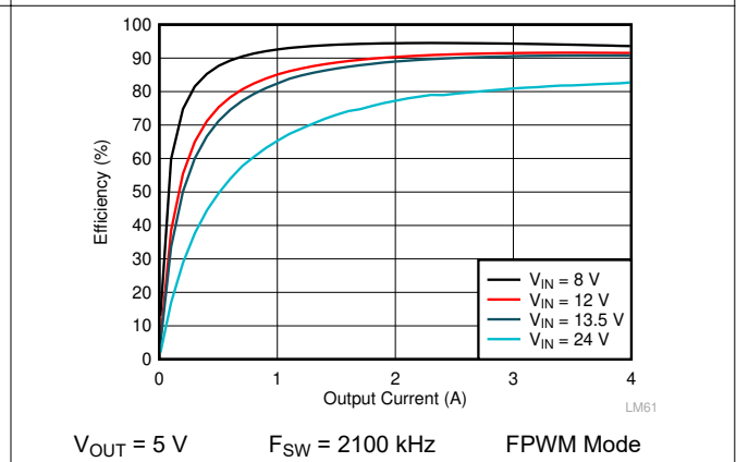
Figure 9-8. LMQ62440-Q1 Efficiency
