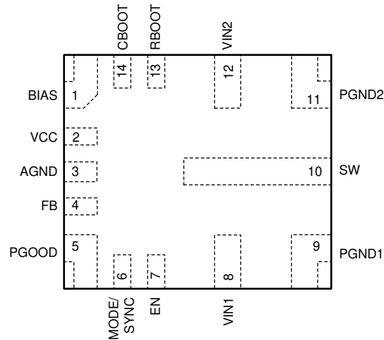
Figure 6-1. RJR Package 14-Pin VQFN-HR Top View
