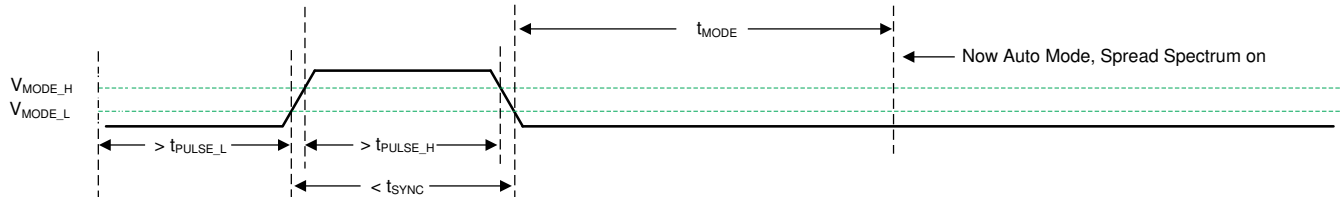
Figure 8-10. Transition from SYNC Mode to Auto Mode
