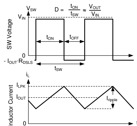
Figure 8-22. SW Voltage and Inductor Current Waveforms in Continuous Conduction Mode (CCM)
