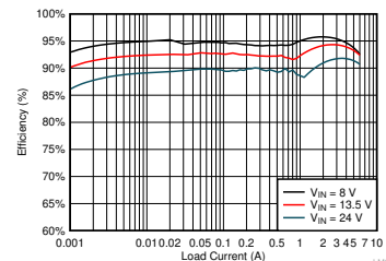
Efficiency: V_{OUT} = 5\text{ V} , F_{SW} = 2.1\text{ MHz}
