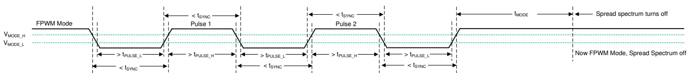
Figure 8-6. Spread Spectrum Disabled in FPWM Mode
