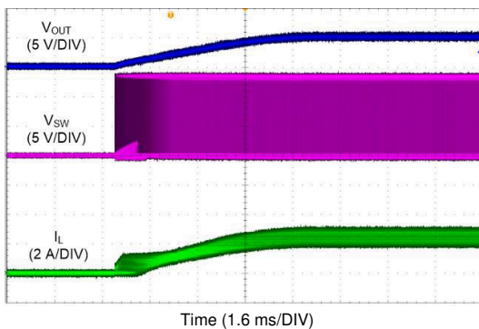
Figure 9-19. LMQ62440-Q1 Start-up with 3.25-A
