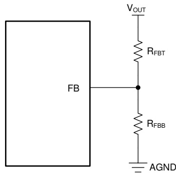
Figure 8-18. Setting Output Voltage of Adjustable Versions
