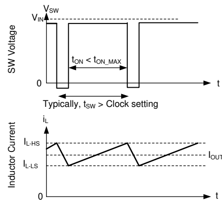
Figure 8-19. Current Limit Waveforms
