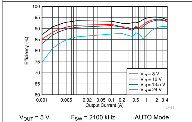
Figure 9-7. LMQ62440-Q1 Efficiency
