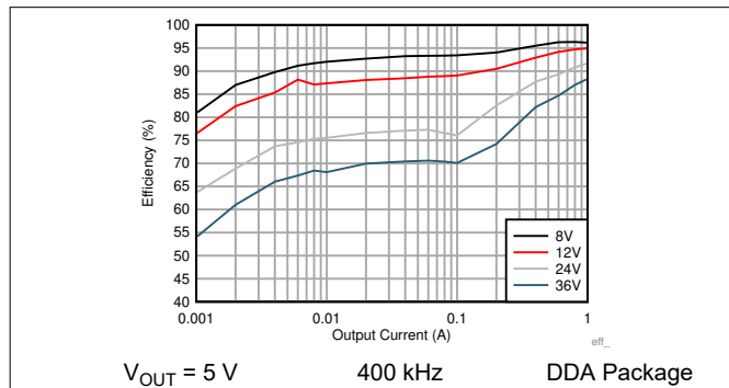
Figure 9-6. Efficiency
