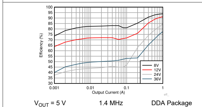
Figure 9-8. Efficiency
