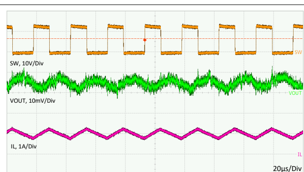
Figure 8-8. Typical PWM Switching Waveforms, V_{IN} = 12\text{ V} , V_{OUT} = 5\text{ V} , I_{OUT} = 1\text{ A} , f_s = 400\text{ kHz}
