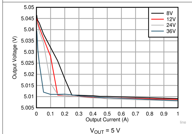
Figure 9-10. Line and Load Regulation
