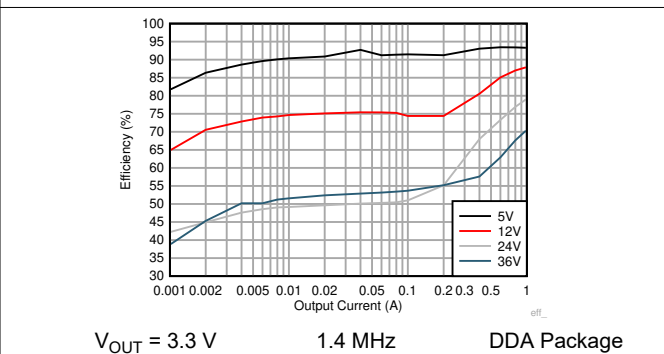
Figure 9-9. Efficiency
