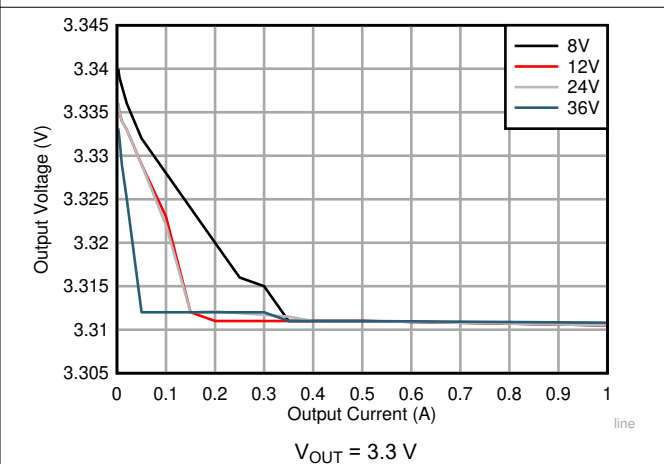
Figure 9-11. Line and Load Regulation
