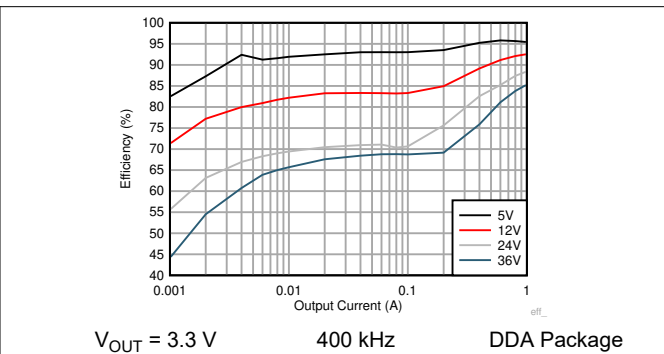
Figure 9-7. Efficiency
