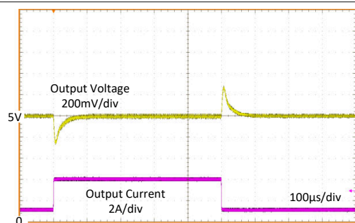
Figure 9-11. Load Transient
