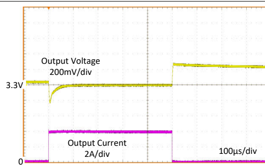
Figure 9-14. Load Transient
