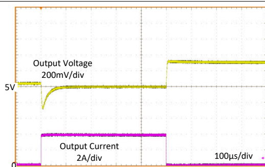
Figure 9-13. Load Transient
