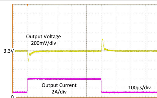
Figure 9-12. Load Transient
