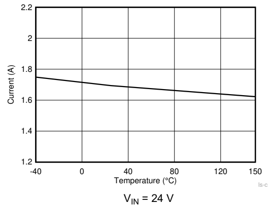
Figure 8-4. Low Side Current Limit
