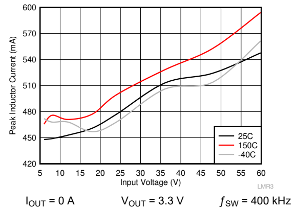
Figure 8-6. I_{PEAK-MIN}
