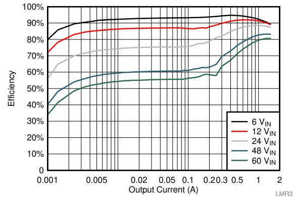
V_{OUT} = 3.3\text{ V} 400 kHz
