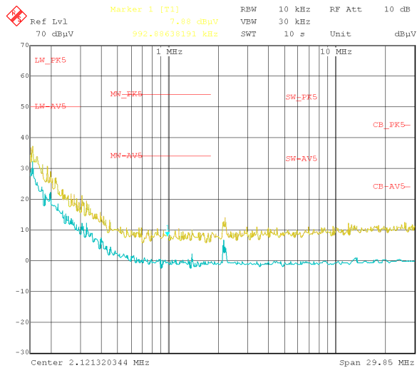
V_{IN} = 13.5\text{ V} V_{OUT} = 5\text{ V} I_{OUT} = 1.5\text{ A} Frequency Tested: 150 kHz to 30 MHz
