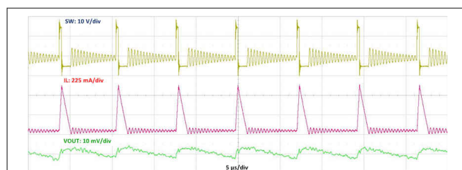
Figure 9-7. Typical PFM Switching Waveforms V_{IN} = 24\text{ V} , V_{OUT} = 5\text{ V} , I_{OUT} = 200\text{ mA}
