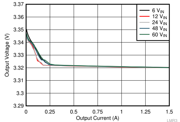
V_{OUT} = 3.3\text{ V} 400 kHz
