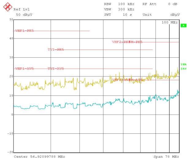
V_{IN} = 13.5\text{ V} V_{OUT} = 5\text{ V} I_{OUT} = 1.5\text{ A} Frequency Tested: 30 MHz to 108 MHz
