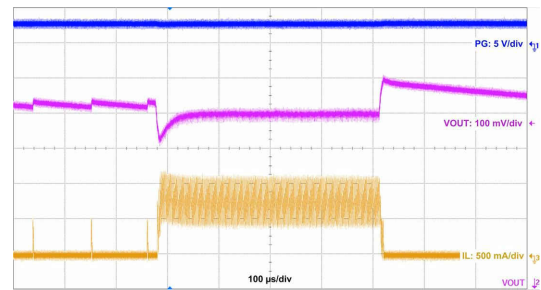
V_{OUT} = 3.3\text{ V} I_{LOAD} = 10\text{ mA} - 0.75\text{ A} 400 kHz Slew Rate = 1\ \mu\text{s/A}
