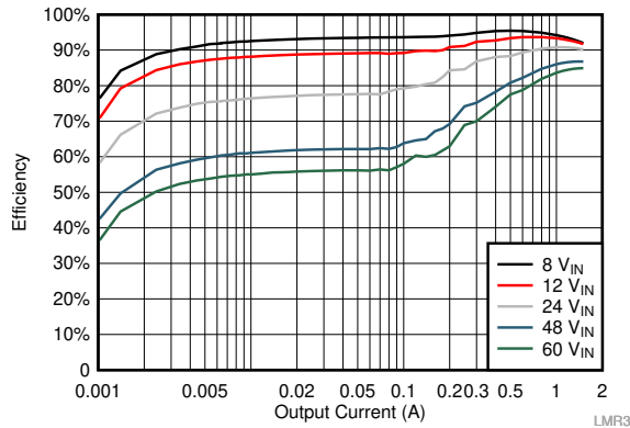
V_{OUT} = 5\text{ V} 400 kHz
