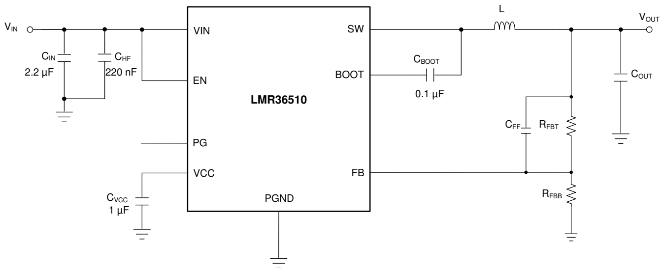
Figure 8-1. Example Applications Circuit
