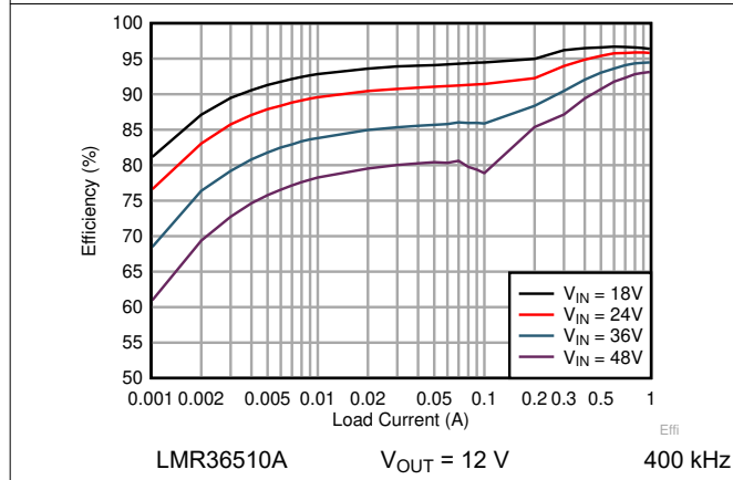
Figure 8-8. Efficiency
