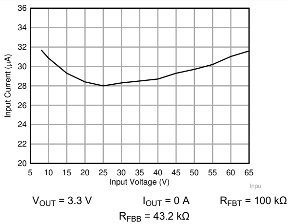
Figure 8-12. Input Supply Current
