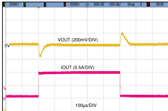
V_{OUT} = 5\text{ V} 400 kHz I_{LOAD} = 0.1\text{ A} - 1\text{ A} Slew Rate = 1 A/ \mu s
