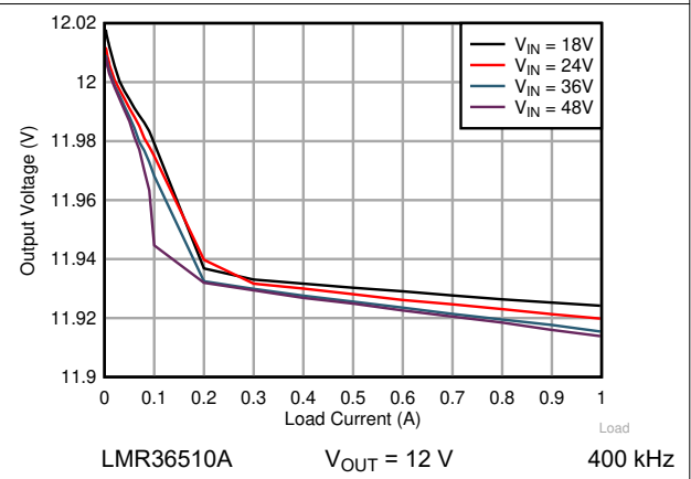
Figure 8-9. Load Regulation
