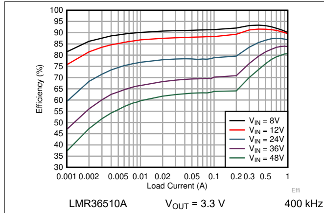
Figure 8-4. Efficiency
