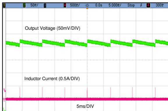
V_{IN} = 24\text{ V} V_{OUT} = 5\text{ V} I_{LOAD} = 0\text{ A}
