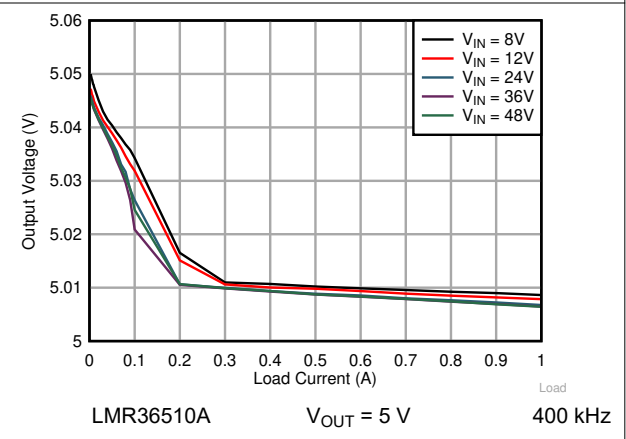
Figure 8-7. Load Regulation
