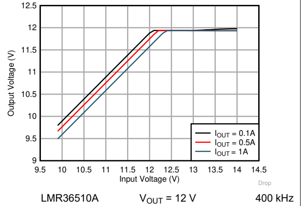
Figure 8-11. Dropout Characteristic
