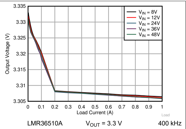
Figure 8-5. Load Regulation
