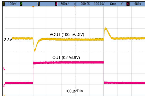
V_{OUT} = 3.3\text{ V} 400 kHz I_{LOAD} = 0.1\text{ A} - 1\text{ A} Slew Rate = 1 A/ \mu s
