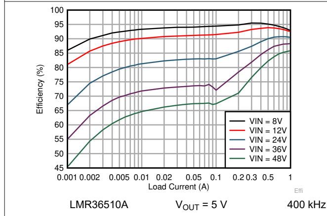
Figure 8-6. Efficiency
