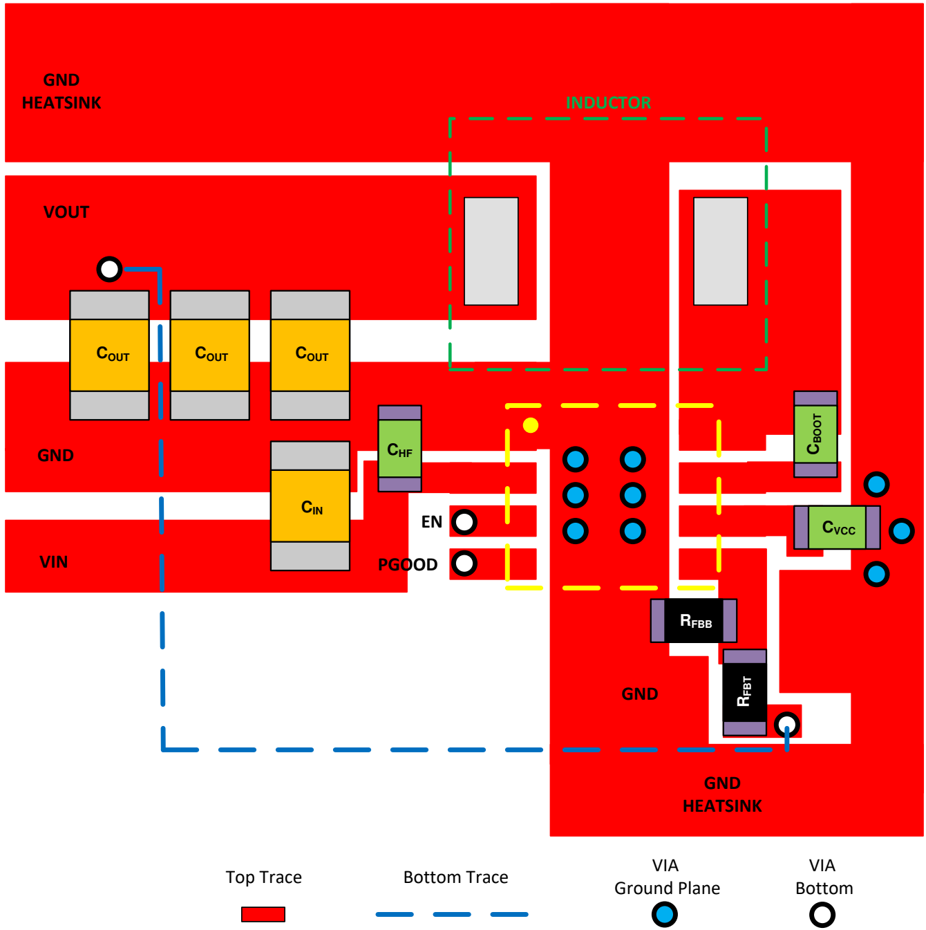
Figure 8-24. Example Layout
