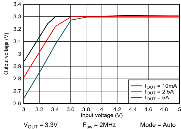
Figure 8-10. Dropout Curve
