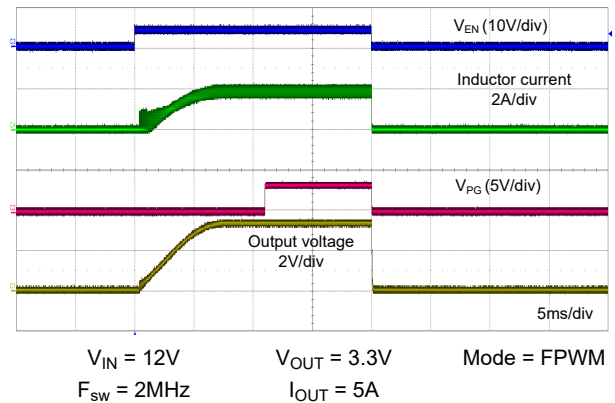
Figure 8-17. Enable Start-Up and Shutdown With 5A Load
