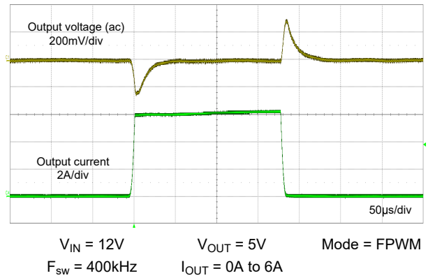
Figure 8-25. Load Transient
