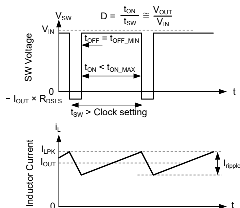
Figure 7-11. Dropout Waveforms
