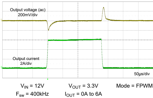
Figure 8-24. Load Transient
