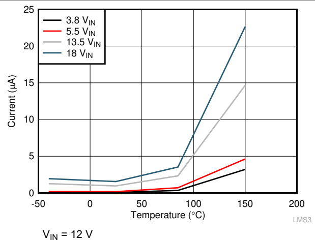
Figure 7-6. Shutdown Current
