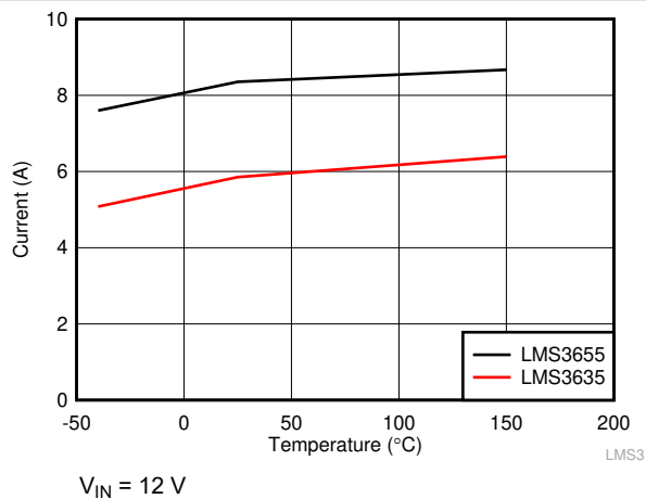
Figure 7-3. High-Side/Peak Current Limit for LMS36x5-Q1
