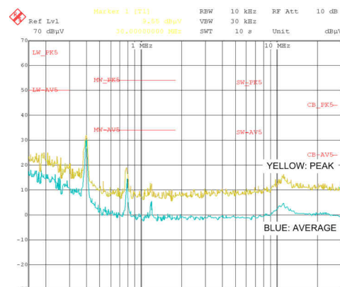
LMS3655-Q1 Conducted EMI: V_{OUT} = 5\text{ V} , I_{OUT} = 5\text{ A}
