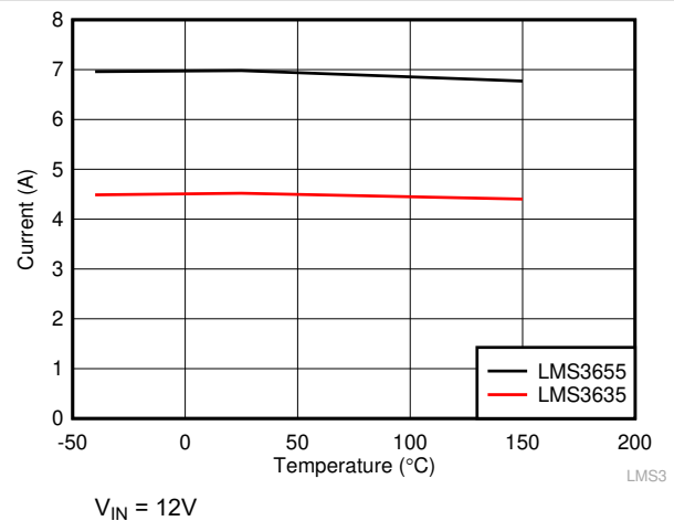
Figure 7-4. Low-Side/Valley Current Limit for LMS36x5-Q1
