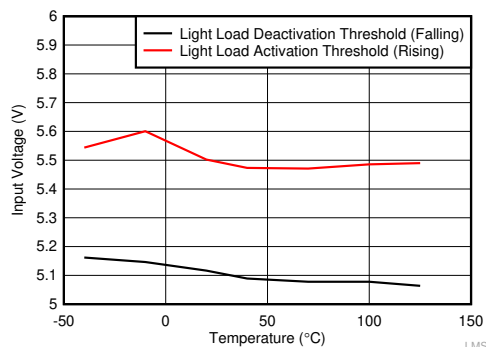
Figure 8-9. Input Voltage for Mode Change — 5-V Output, 10-μH Inductor
