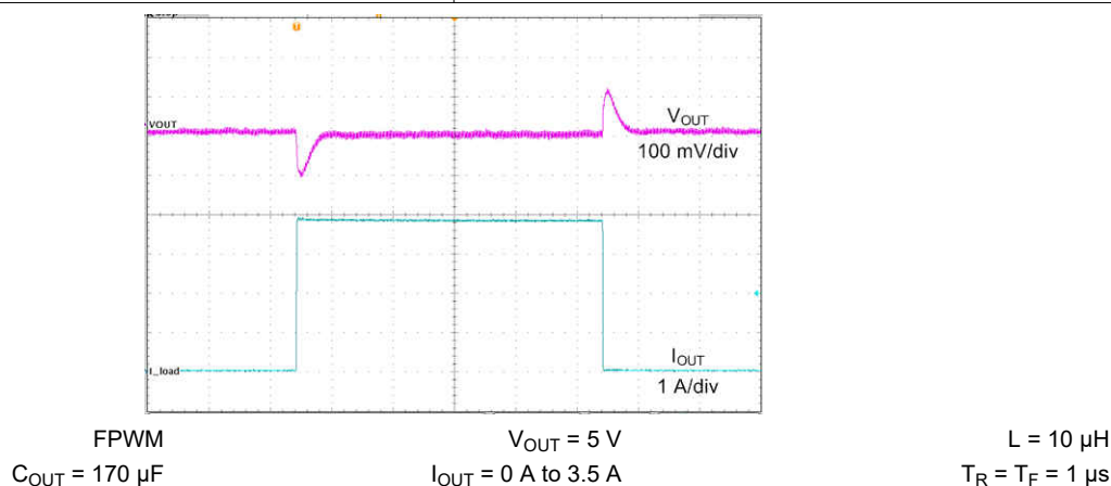
Figure 9-15. Load Transient
