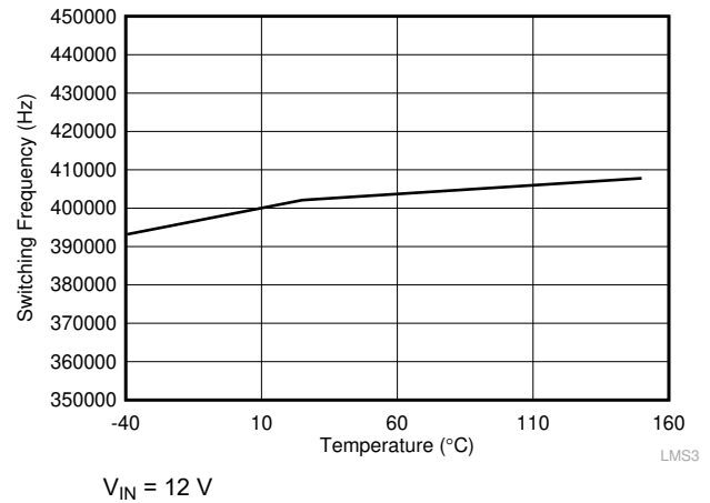
Figure 7-2. Switching Frequency vs Temperature
