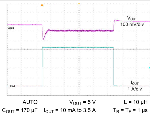
Figure 9-14. Load Transients
