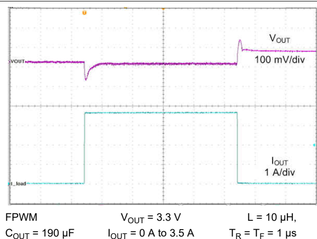
Figure 9-28. Load Transient
