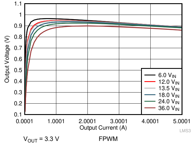
Figure 9-18. Efficiency
