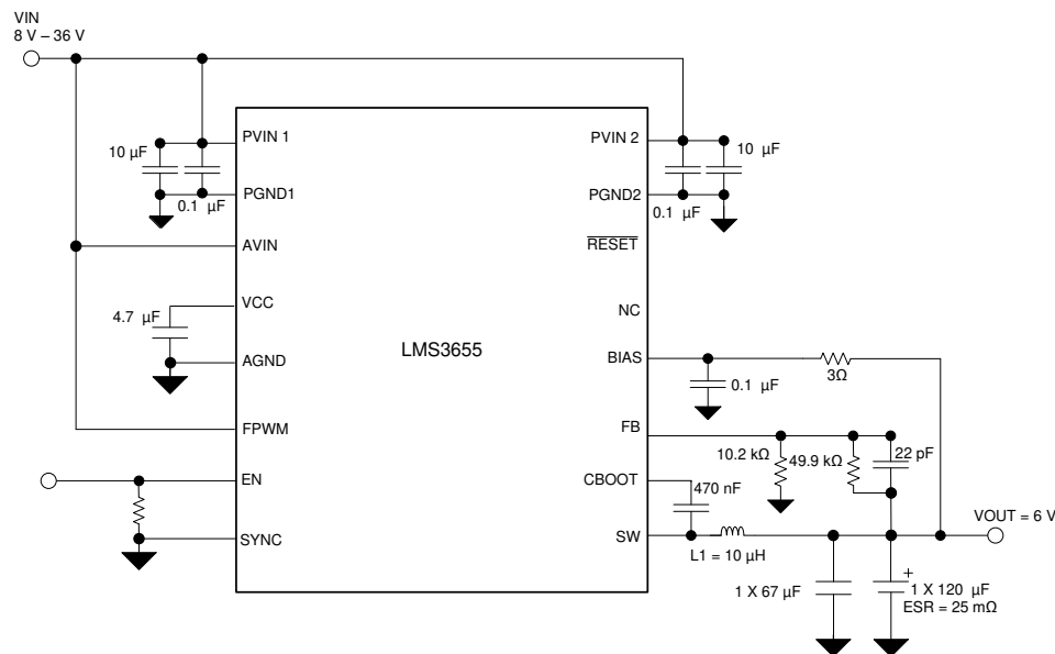
Figure 9-30. 6-V Output Power Supply
