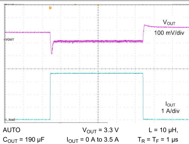
Figure 9-27. Load Transient
