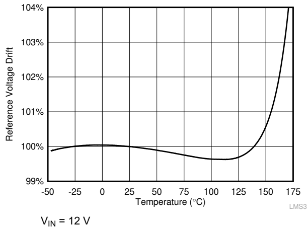
Figure 7-1. Reference Voltage Drift
