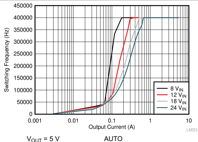
Figure 9-12. Switching Frequency vs Load Current
