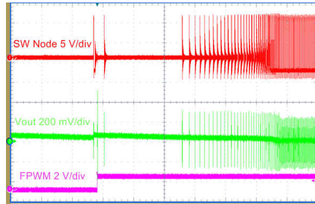
Figure 9-29. Mode Change Transient AUTO to FPWM mode
