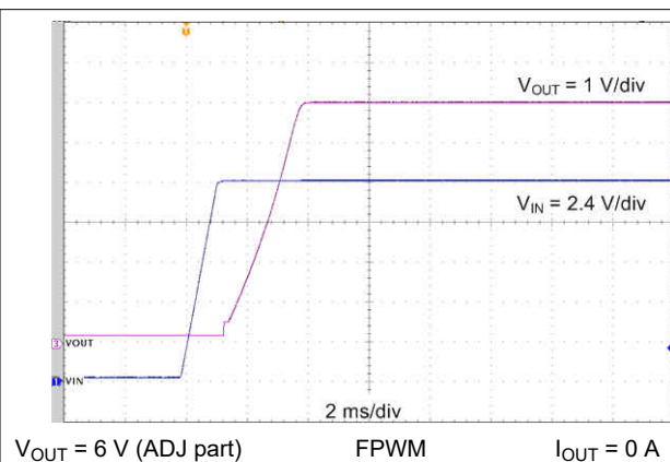
Figure 9-32. Start-Up Waveform (EN Tied to VIN)
