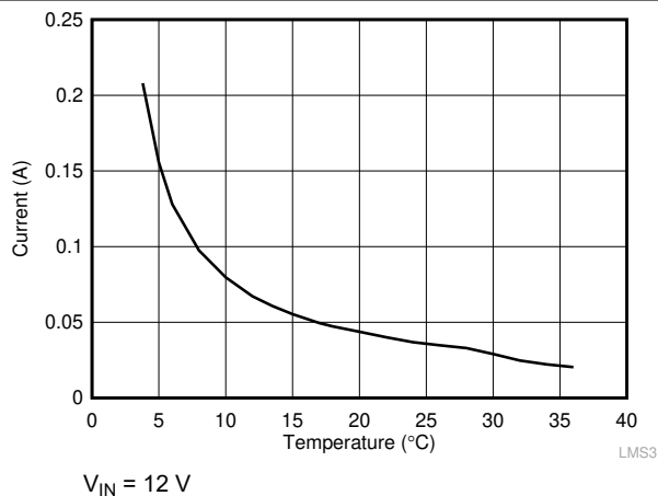
Figure 7-5. Short Circuit Average Input Current for LMS3635-Q1
