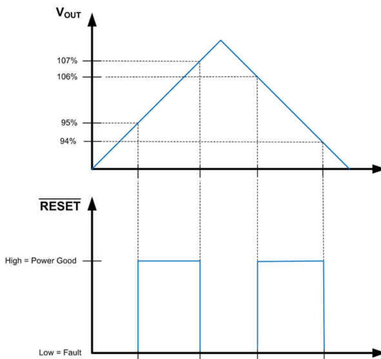
Figure 8-2. Static \overline{RESET} Operation
