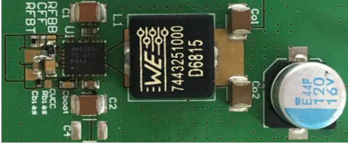
Figure 11-3. LMS3655MQEVM Layout
