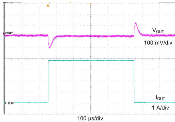
Figure 9-33. Load Transient
