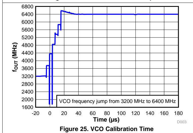
f_{\text{VCO}} = 6397 \text{ MHz} ; f_{\text{PD}} = 100 \text{ MHz} ; 3 rd order modulator; Fractional denominator = 1000; Loop filter bandwidth = 115 kHz
