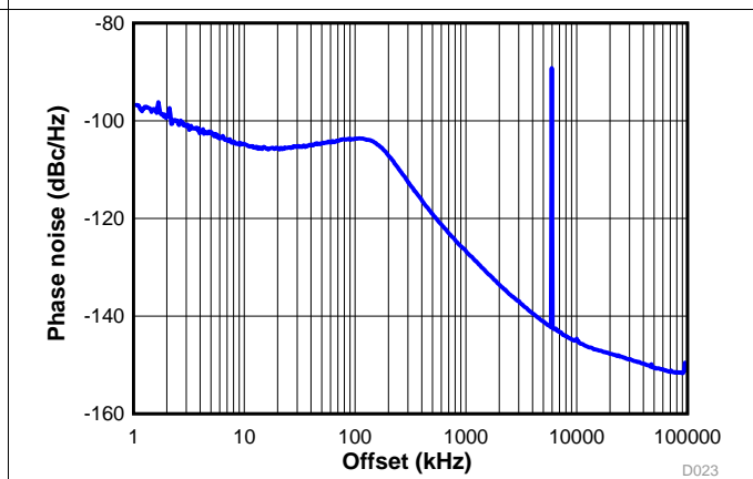
f_{\text{VCO}} = 6397 \text{ MHz} ; f_{\text{PD}} = 100 \text{ MHz} ; 3 rd order modulator; Fractional denominator = 2^{32} - 1 ; Loop filter bandwidth = 115 kHz
