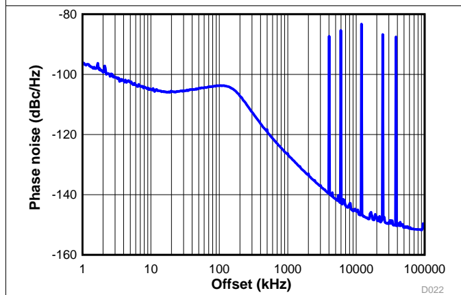
f_{\text{VCO}} = 6397 \text{ MHz} ; f_{\text{PD}} = 100 \text{ MHz} ; 3 rd order modulator; Fractional denominator = 1000; Loop filter bandwidth = 115 kHz
