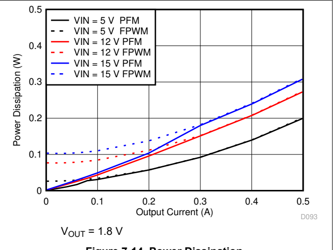
Figure 7-14. Power Dissipation
