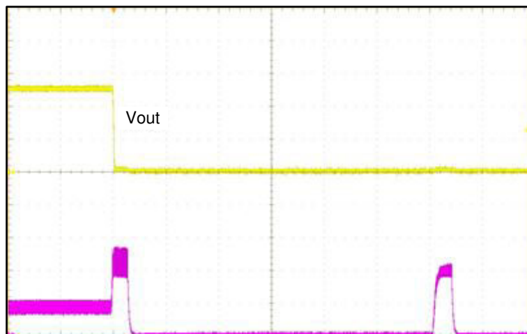
Figure 8-2. Hiccup Operation
