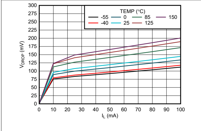
Figure 5-9. Dropout Voltage ( V_{DO} ) vs Load Current (New Chip)
