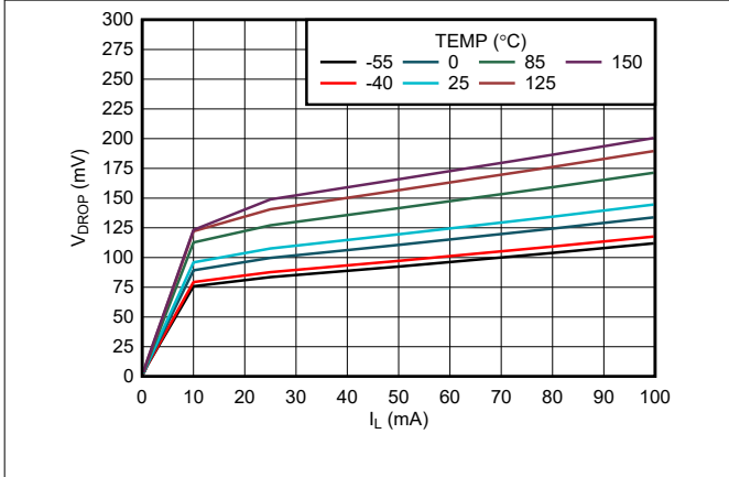
Figure 5-9. Dropout Voltage ( V_{DO} ) vs Load Current (New Chip)
