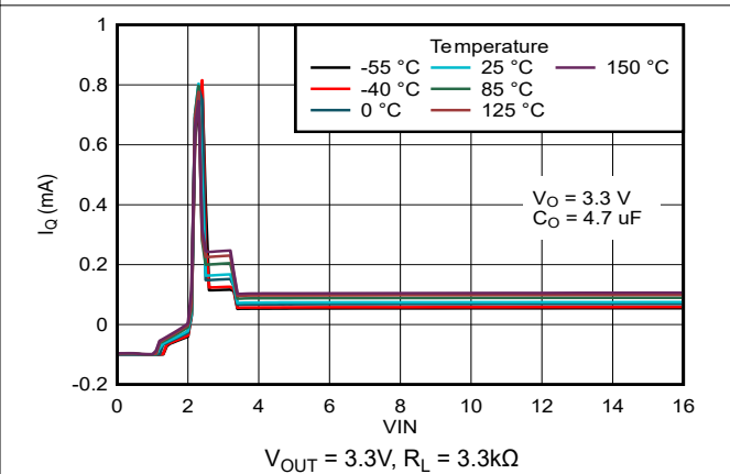
Figure 5-12. Input Current vs Input Voltage ( V_{IN} ) (New Chip)
