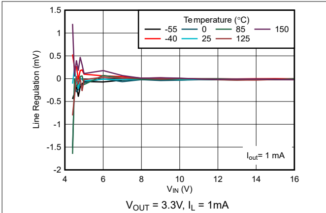
Figure 5-7. Line Regulation vs V_{IN} and Temperature (New Chip)
