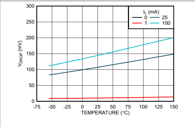
Figure 5-8. Dropout Voltage ( V_{DO} ) vs Temperature (New Chip)
