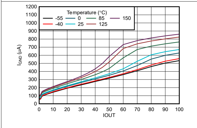
Figure 5-11. Ground Pin Current ( I_{GND} ) vs Load Current (New Chip)
