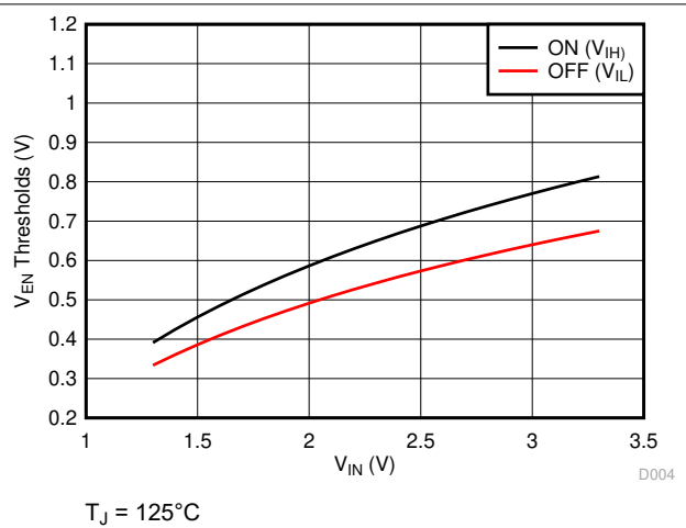
Figure 6-2. V_{EN} Thresholds vs V_{IN}
