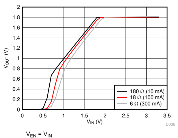
Figure 6-6. V_{OUT} vs V_{IN}
