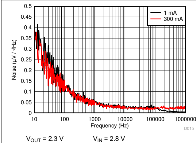
Figure 6-15. Noise Density
