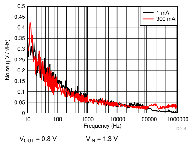
Figure 6-14. Noise Density
