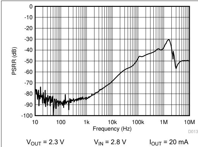
Figure 6-13. PSRR vs Frequency
