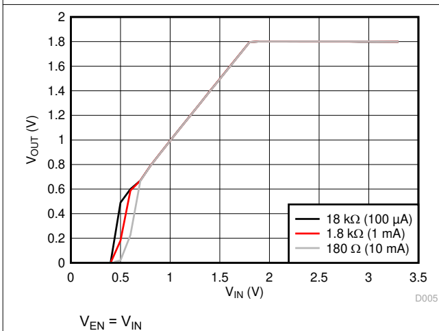
Figure 6-5. V_{OUT} vs V_{IN}
