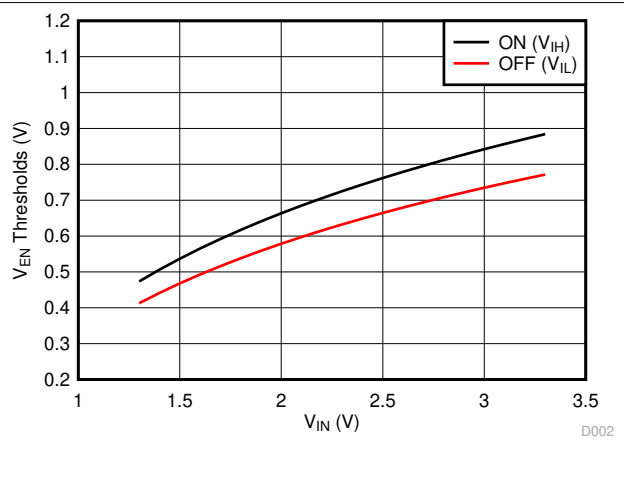
Figure 6-2. V_{EN} Thresholds vs V_{IN}
