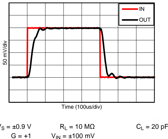
Figure 27. Pulse Response, 200mVpp at 1.8 V
