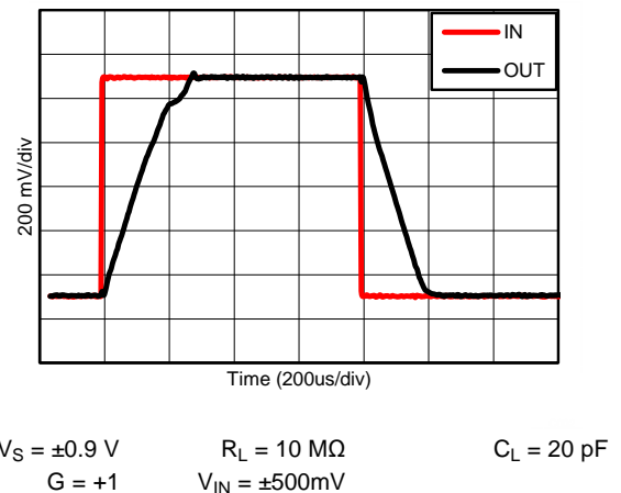
Figure 28. Pulse Response, 1Vpp at 1.8V
