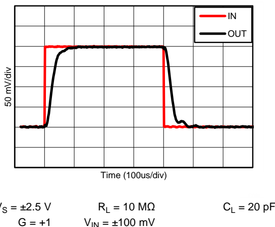
Figure 29. Pulse Response, 200mVpp at 5V
