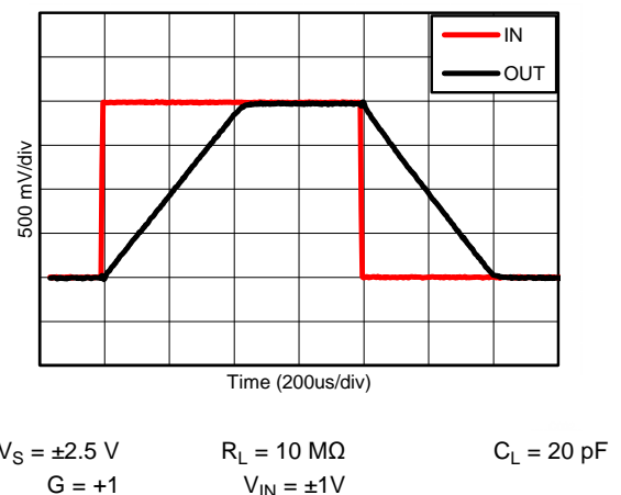
Figure 30. Pulse Response, 2Vpp at 5V
