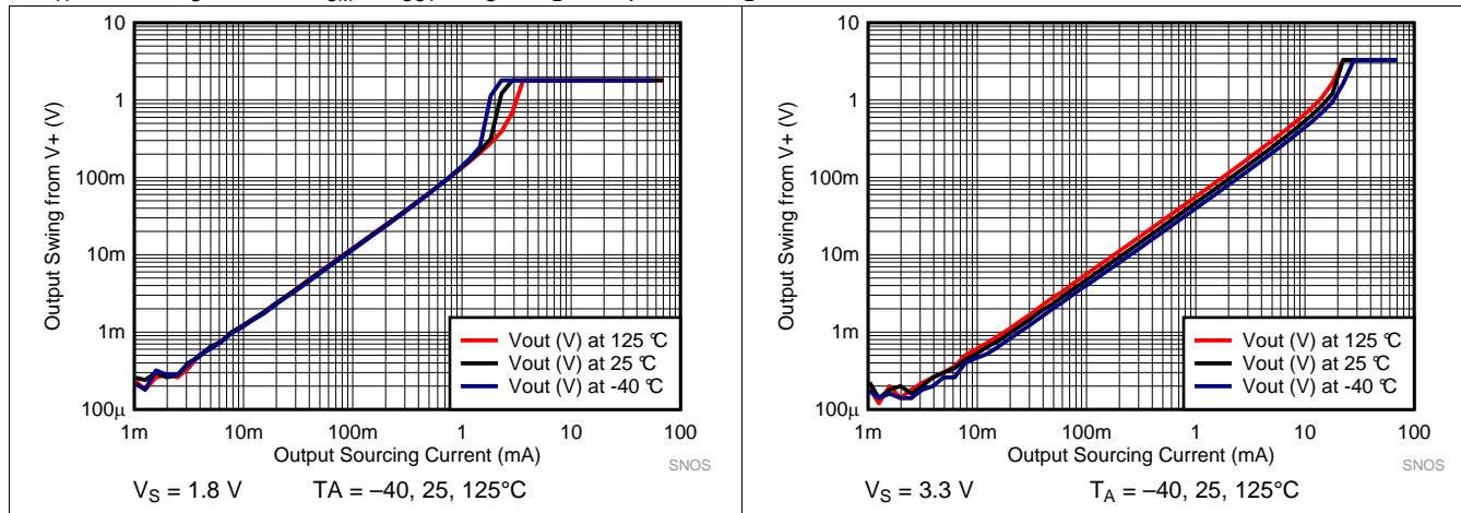
Figure 31. Output Swing vs Sourcing Current, 1.8 V
