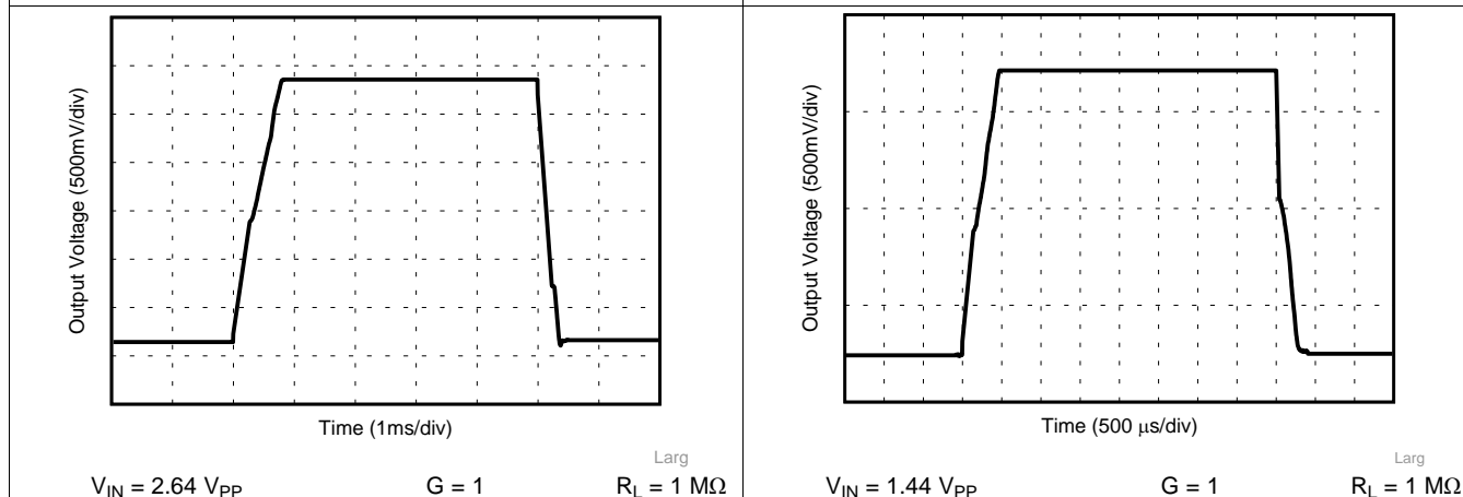
Figure 33. Large-Signal Response, 3.3V
