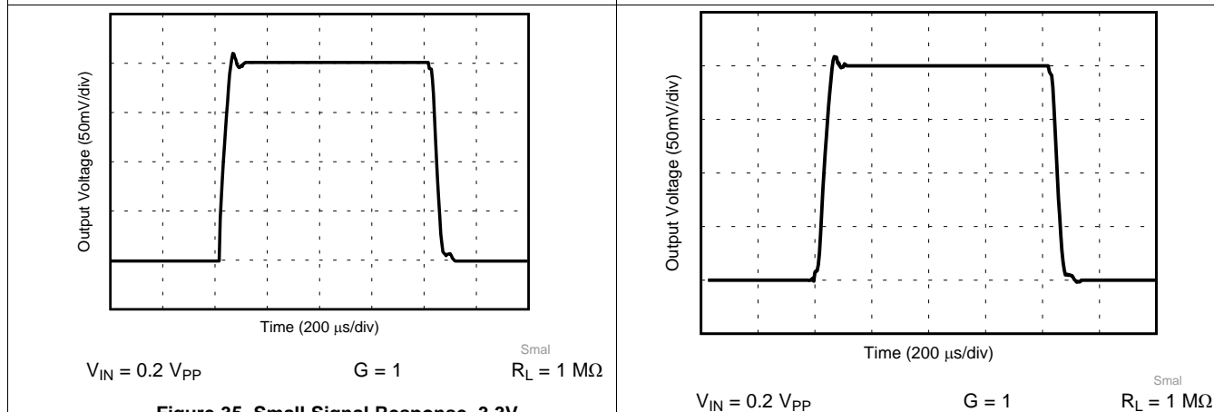
Figure 35. Small Signal Response, 3.3V
