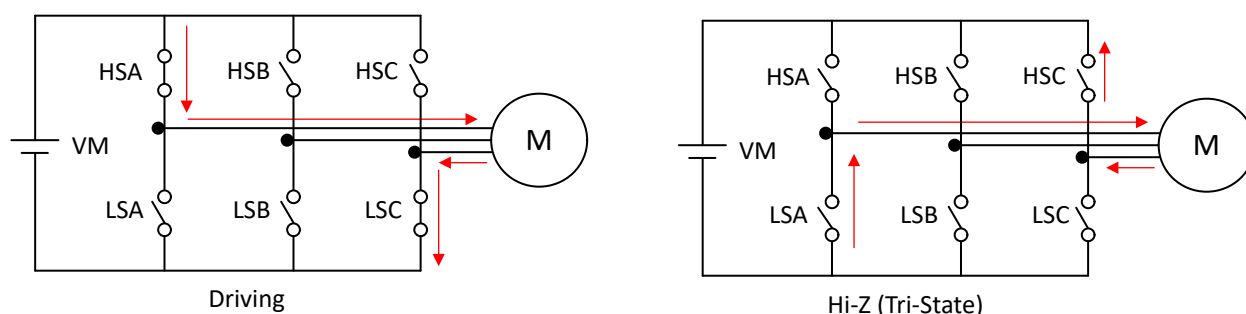
Figure 6-19. IPD Release Hi-Z mode
