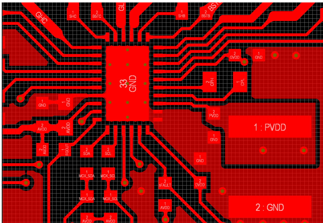
Figure 9-6. Layout example of MCF8329A-Q1
