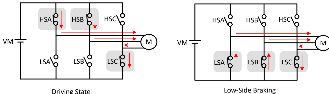
Figure 6-40. Low-Side Braking
