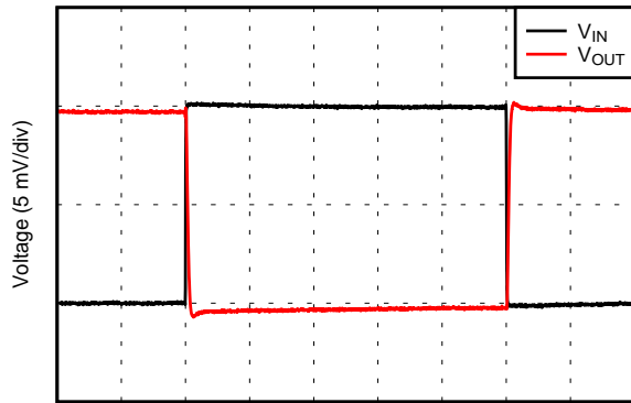
Figure 33. Positive Overload Recovery
