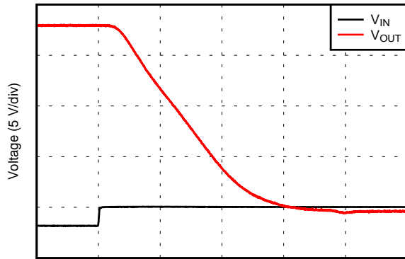
Figure 31. Normalized Settling Time
