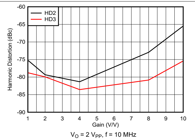
Figure 7-41. Harmonic Distortion vs Noninverting Gain
