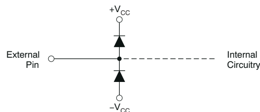
Figure 9-3. ESD Steering Diodes
