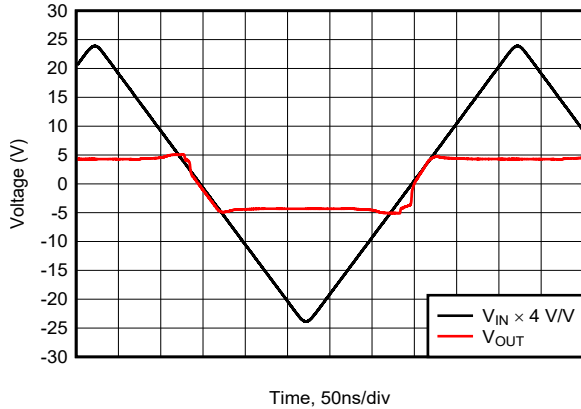
Figure 7-7. Overdrive Recovery
