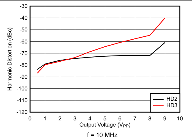
Figure 7-39. Harmonic Distortion vs Output Voltage
