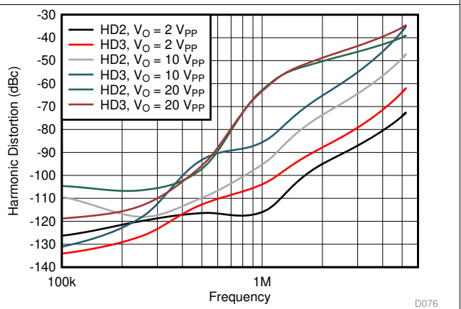
See Figure 64, Gain = 2 V/V
