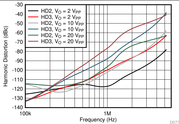
See Figure 65, Gain = -1 V/V
