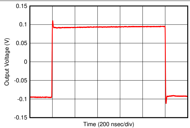
See Figure 64, Gain = 1 V/V, R_F = 0\ \Omega
