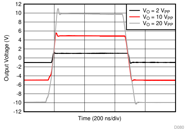
See Figure 64, Gain = 2 V/V
