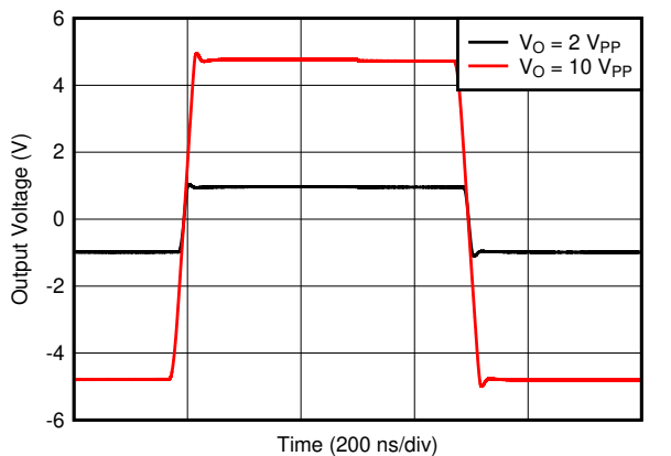
See Figure 65, Gain = -1 V/V
