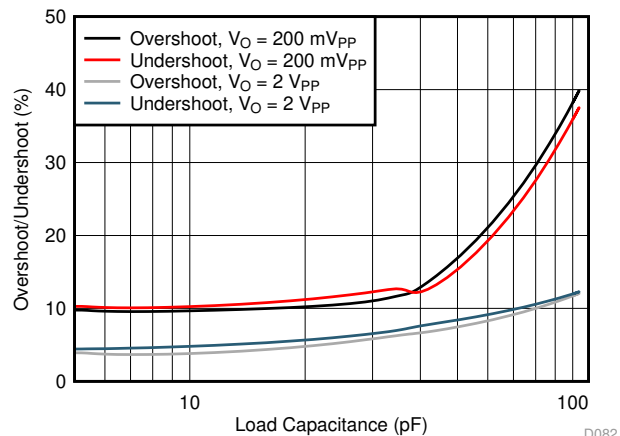
See Figure 64, Gain = 1 V/V, R_F = 0\ \Omega
