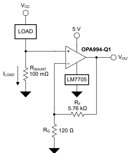
Figure 7-1. OPA994-Q1 in a Low-Side, Current-Sensing Application
