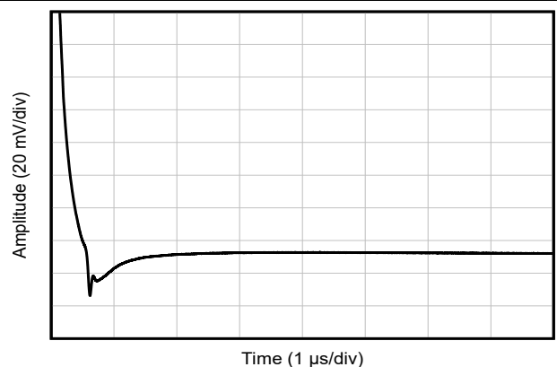
Figure 5-48. Settling Time
