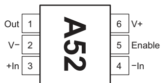
Figure 4-1. OPA300, SOT-23 Package, 6-pin (Top View)
