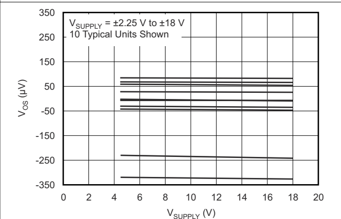
Figure 6-6. Offset Voltage vs Power Supply
