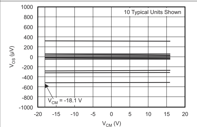
Figure 6-4. Offset Voltage vs Common-Mode Voltage: V_{\text{SUPPLY}} (V) = \pm 18 V
