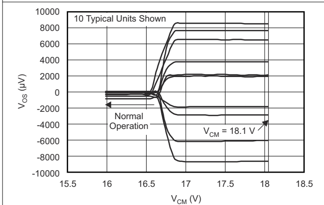
Figure 6-5. Offset Voltage vs Common-Mode Voltage: V_{\text{SUPPLY}} (V) = \pm 18 V (Upper Stage)
