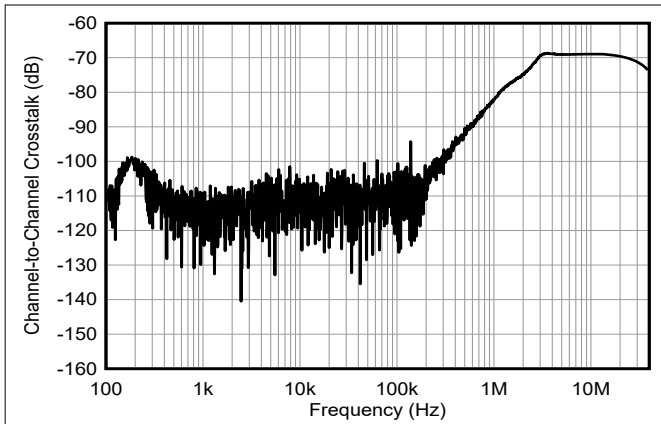
Figure 5-19. Channel-to-Channel Crosstalk
