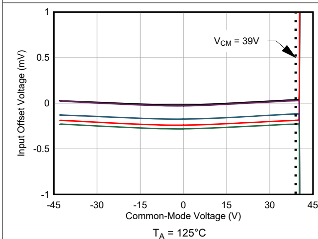
Figure 5-5. Input Offset Voltage vs Common-Mode Voltage
