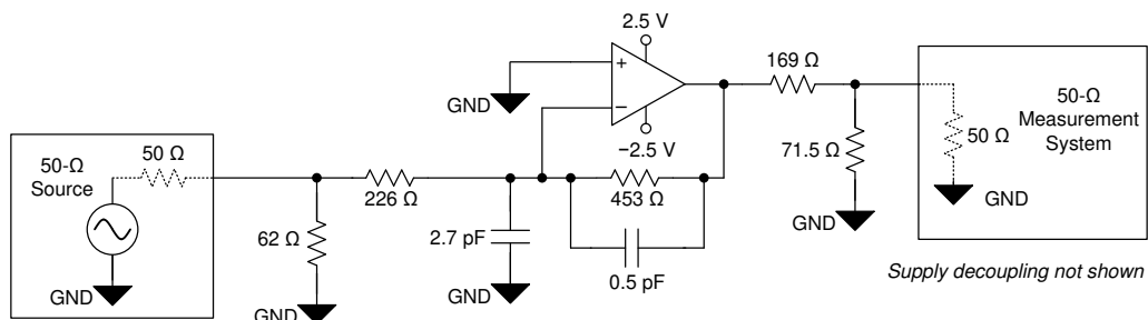
Figure 9-5. OPA858 in a Gain of -2V/V (With Noise Gain Shaping)
