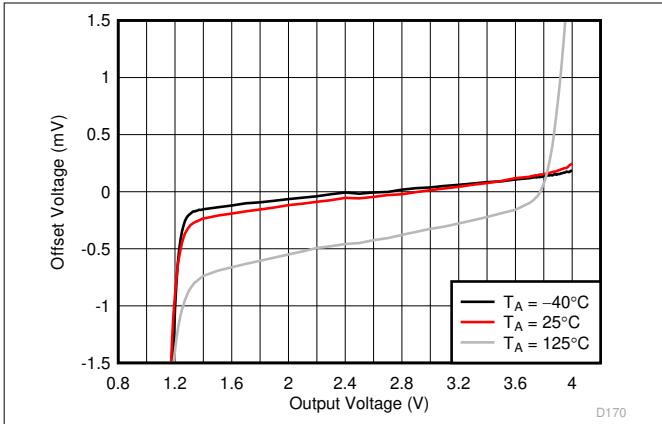
Figure 6-37. Offset Voltage vs Output Swing vs Ambient Temperature
