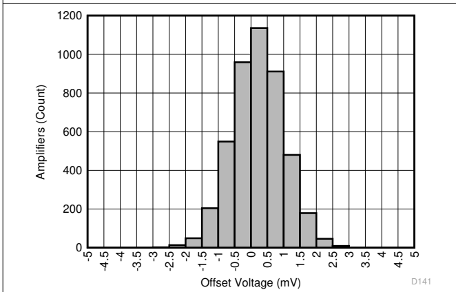
\mu = -0.28\text{ mV} \sigma = 0.8\text{ mV} 4555 units tested
