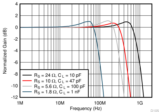
V_{OUT} = 100\text{ mV}_{PP} ; see Figure 7-3 for circuit configuration
