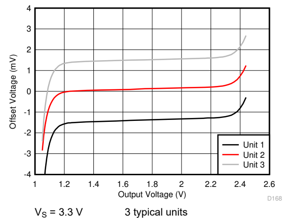
Figure 6-35. Offset Voltage vs Output Swing
