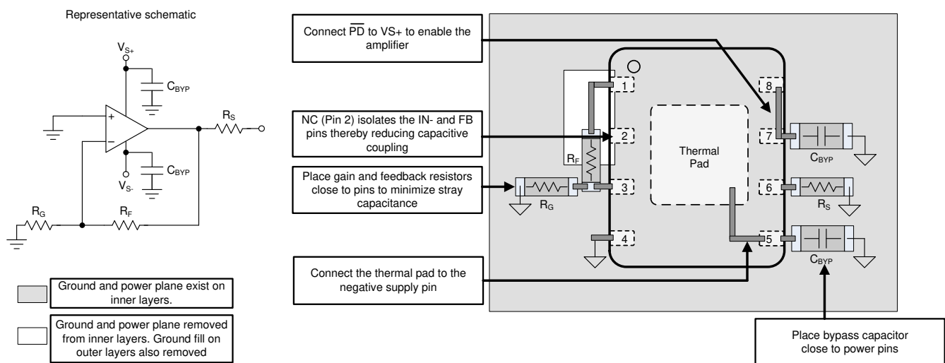
Figure 9-9. Layout Recommendation
