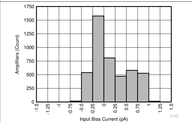
\mu = -0.1\text{ pA} \sigma = 0.39\text{ pA} 4555 units tested
