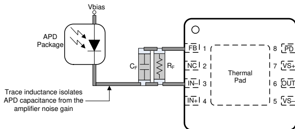
Figure 9-10. Nonideal TIA Layout
