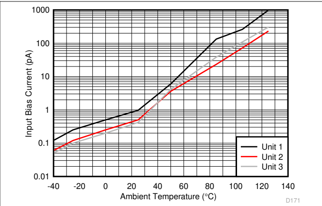
Figure 6-38. Input Bias Current vs Ambient Temperature
