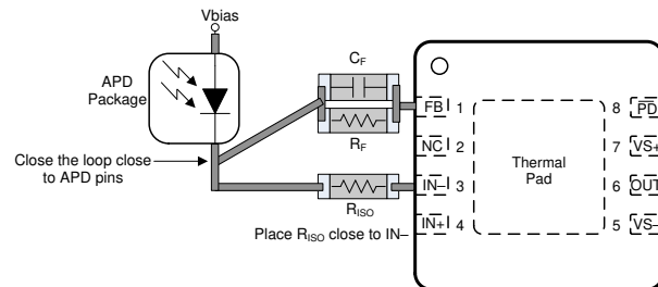
Figure 9-11. Improved TIA Layout
