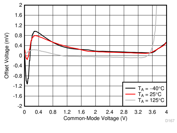
Figure 6-34. Offset Voltage vs Input Common-Mode Voltage vs Ambient Temperature
