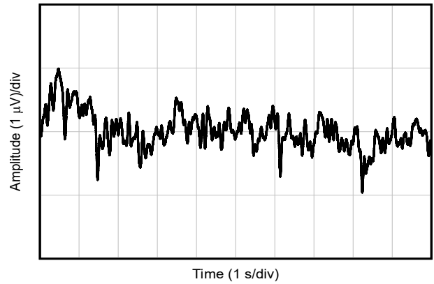
Figure 5-26. 0.1Hz to 10Hz Noise
