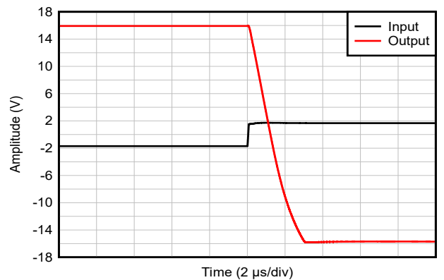
Figure 5-42. Positive Overload Recovery
