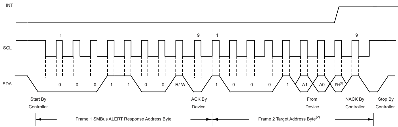
Figure 8-4. Timing Diagram for SMBus Alert Response
