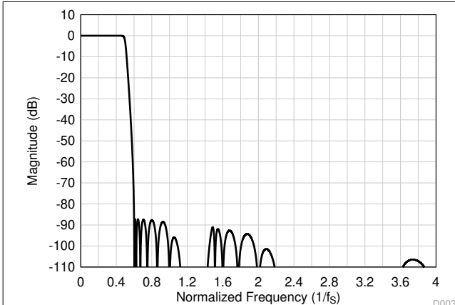
Figure 7-51. Ultra-Low-Latency Decimation Filter Magnitude Response
