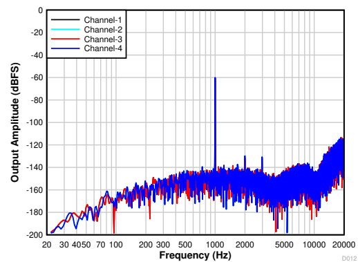
4th-order PDM modulator with \text{PDMCLK}_x = 1.536\text{ MHz} Figure 6-15. FFT With a -60-dBr Input
