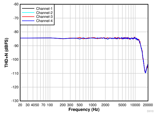
4th-order PDM modulator with \text{PDMCLK}_x = 1.536\text{ MHz} Figure 6-13. THD+N vs Input Frequency With a -20-dBr Input
