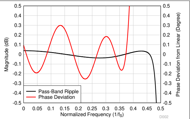
Figure 7-46. Low-Latency Decimation Filter Pass-Band Ripple and Phase Deviation
