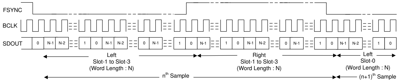
Figure 7-7. I 2 S Protocol Timing (No Idle BCLK Cycles, TX_OFFSET = 0)
