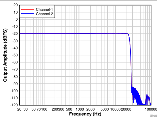
4th-order PDM modulator with \text{PDMCLKx} = 6.144\text{ MHz}
