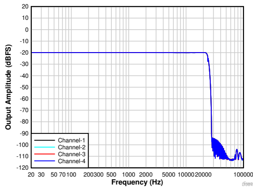
4th-order PDM modulator with \text{PDMCLK}_x = 3.072\text{ MHz} Figure 6-10. Frequency Response With a -20-dBr Input
