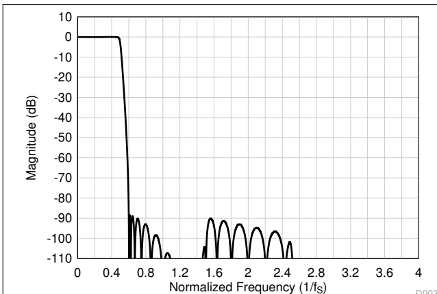
Figure 7-53. Ultra-Low-Latency Decimation Filter Magnitude Response
