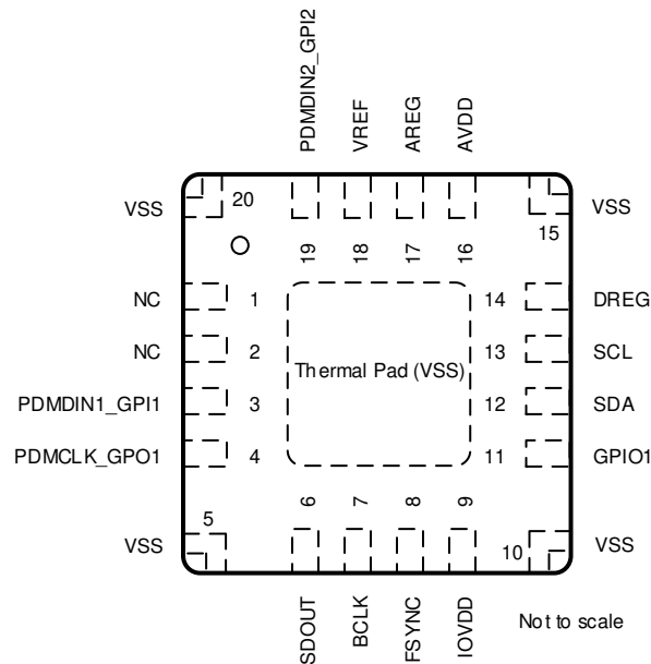
Figure 5-1. RTE Package, 20-Pin WQFN With Exposed Thermal Pad, Top View
