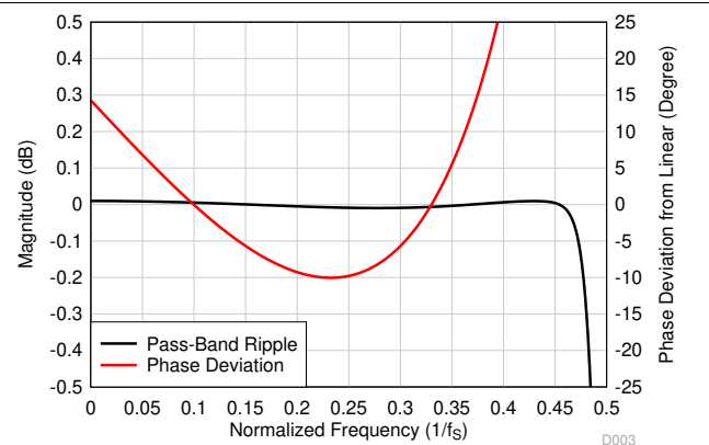
Figure 7-52. Ultra-Low-Latency Decimation Filter Pass-Band Ripple and Phase Deviation
