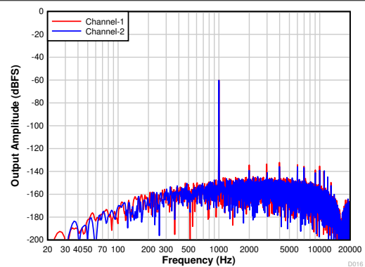
4th-order PDM modulator with \text{PDMCLKx} = 6.144\text{ MHz}
