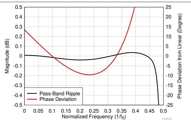
Figure 7-54. Ultra-Low-Latency Decimation Filter Pass-Band Ripple and Phase Deviation
