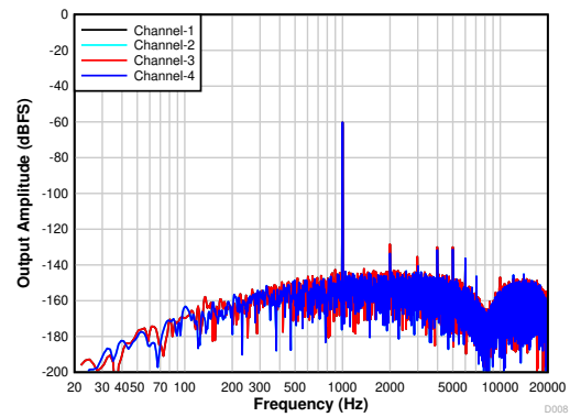
4th-order PDM modulator with \text{PDMCLK}_x = 3.072\text{ MHz} Figure 6-11. FFT With a -60-dBr Input
