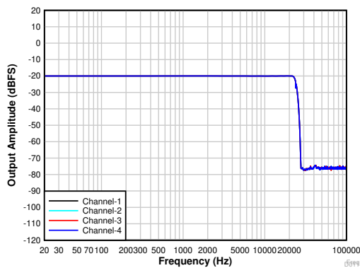
4th-order PDM modulator with \text{PDMCLK}_x = 1.536\text{ MHz} Figure 6-14. Frequency Response With a -20-dBr Input
