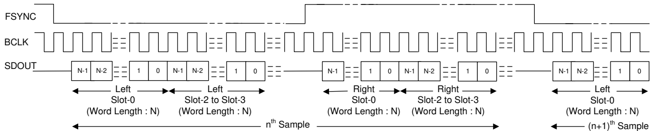
Figure 7-8. I 2 S Protocol Timing (TX_OFFSET = 0 and BCLK_POL = 1)
