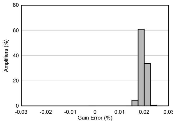
N = 7295 Mean = 0.0195 % Std. dev. = 0.0012 % G = 1 V/V
