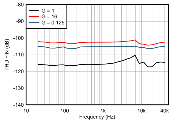
Figure 7-54. Total Harmonic Distortion + Noise vs Frequency 10-Hz to 22-kHz band-pass filter V_{OUTDIFF} > 2.5\text{ V}_{PP}
