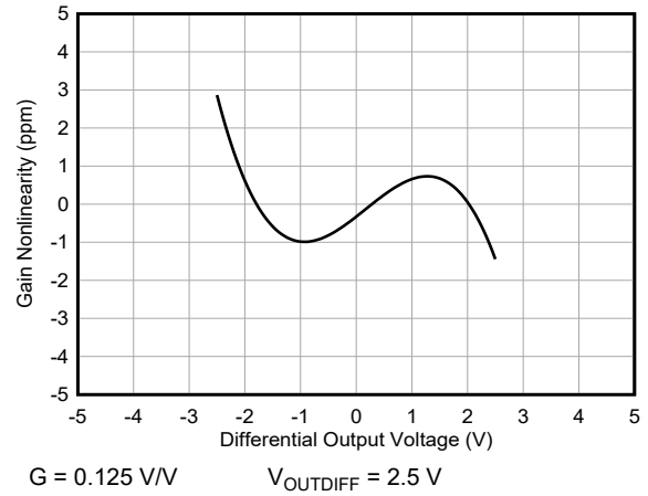
Figure 7-34. Gain Nonlinearity
