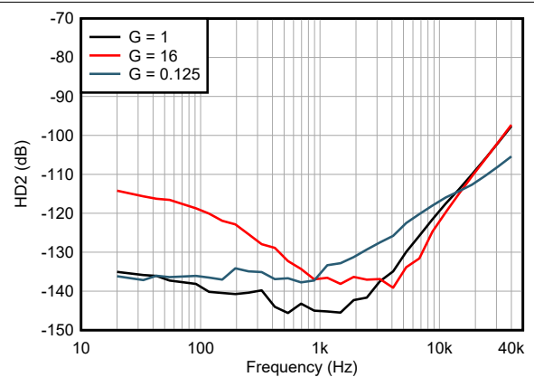
Figure 7-56. 2nd Harmonic Distortion vs Frequency V_{OUTDIFF} > 2.5\text{ V}_{PP}
