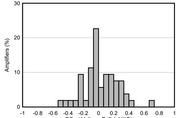
N = 53 Mean = -0.024 \mu\text{V}/^\circ\text{C} Std. dev. = 0.22 \mu\text{V}/^\circ\text{C} G = 1 V/V
