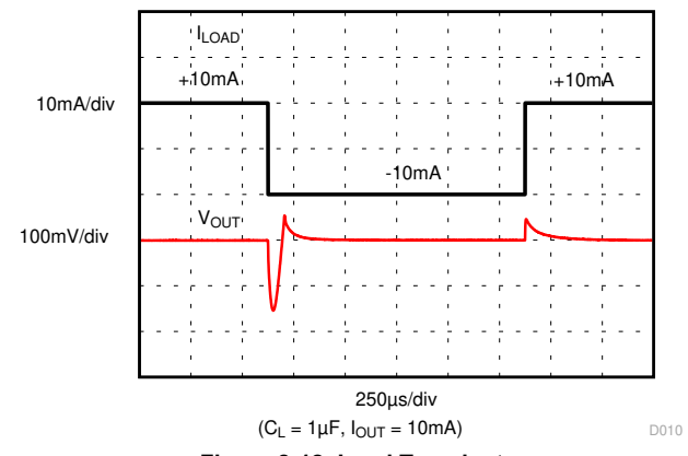
Figure 8-12. Load Transient
