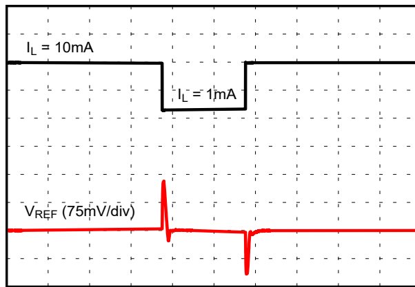
Figure 8-4. Load Transient Response 1mA to 10mA, C_L = 1\mu F
