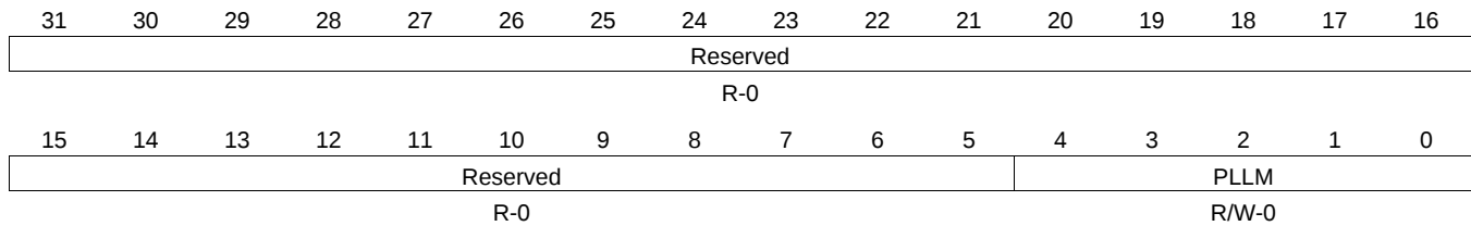
Figure 4-17. PLL Multiplier Control Register (PLLM) (Address - 029A 0110h)
