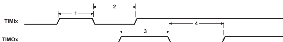
Figure 4-61. Timer Timing
