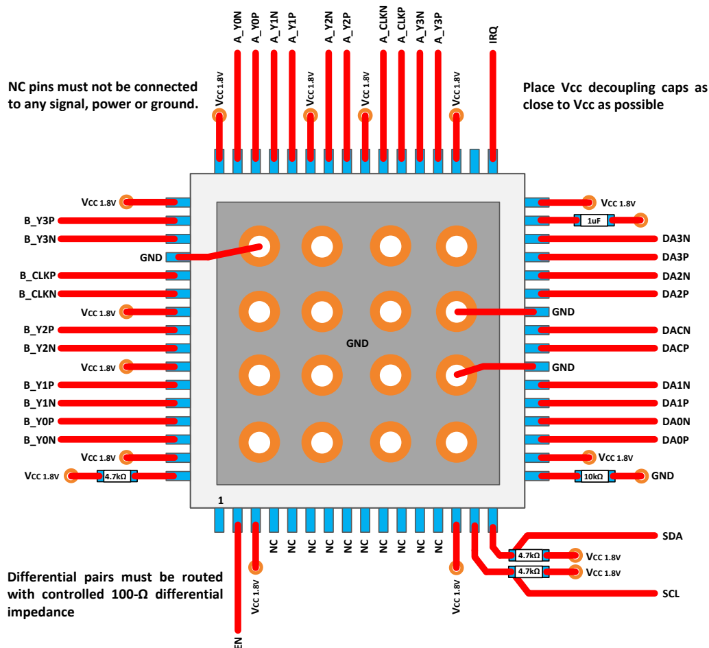
Figure 50. SN65DSI84-Q1 Layout Example
