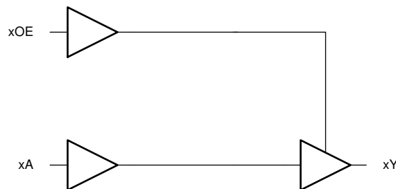
Simplified Schematic
