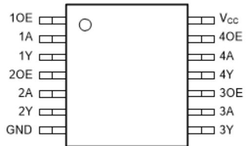
Figure 4-2. SN74AC126-Q1, PW Package (Top View)
