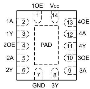
Figure 4-1. SN74AC126-Q1 BQA Package (Top View)
