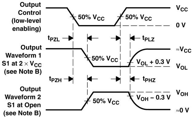
VOLTAGE WAVEFORMS
