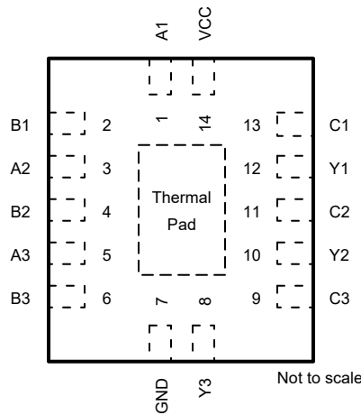
Figure 4-1. SN74AC3G97 BQA Package, 14-Pin WQFN (Top View)
