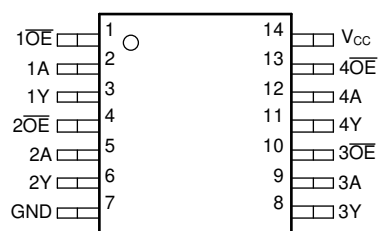
Figure 4-2. SN74ACT125-Q1, PW Package (Top View)
