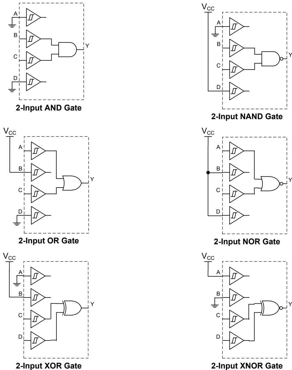
Figure 7-3. Logic Configurations
