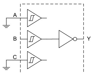
Schmitt-trigger inverter
