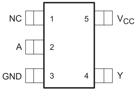
Figure 4-1. DBV Package 5-Pin SOT-23 Top View
