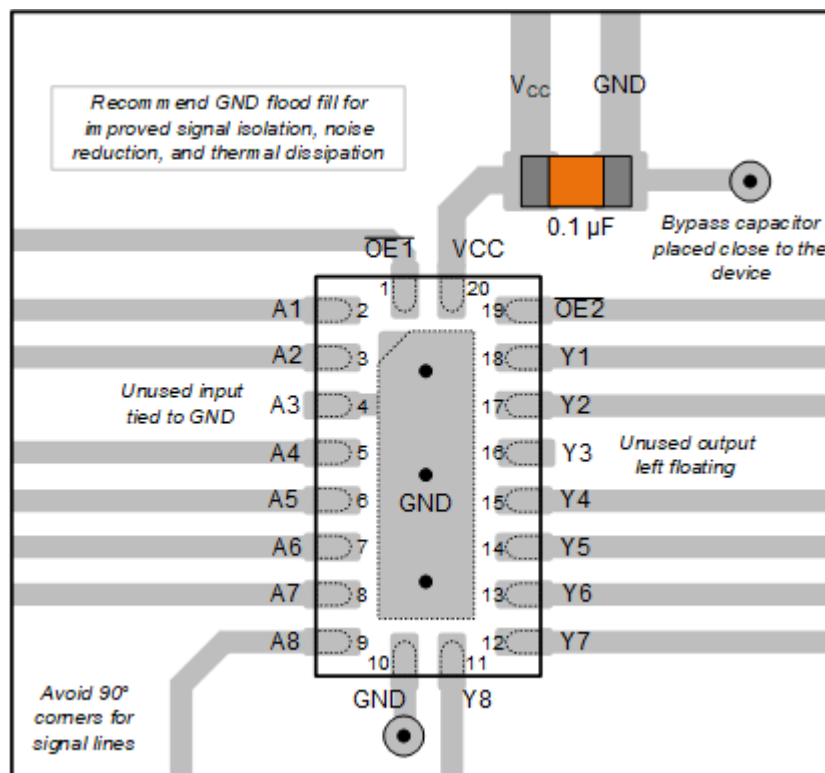
Figure 8-1. Layout Diagram
