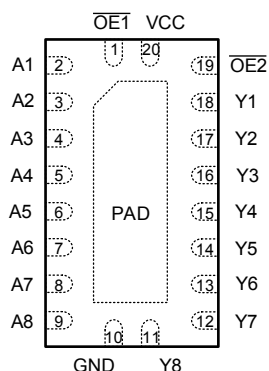
Figure 4-1. SN74AHC7541-Q1 RKS Package (Top View)
