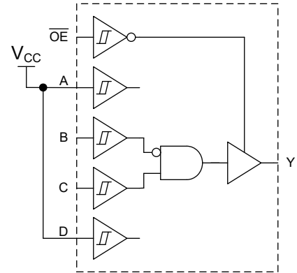
2-Input AND with 1 inverted input
