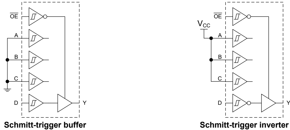
Figure 7-1. Logic Configurations
