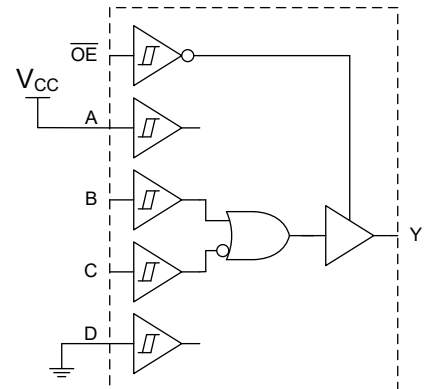
2-Input OR with 1 inverted input
