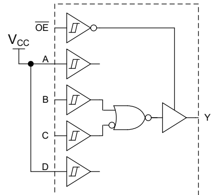
2-Input NOR with 1 inverted input
