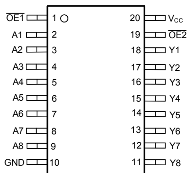
Figure 4-2. SN74AHCT9541-Q1 PW, DGS Package (Top View)
