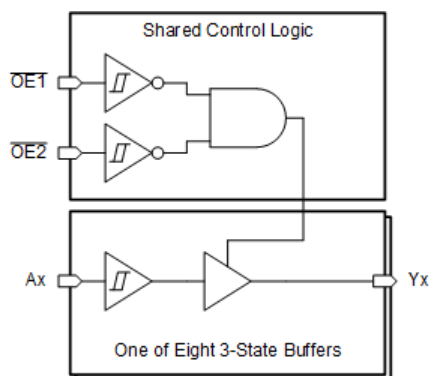
Figure 7-1. Schmitt-trigger Input Diagram
