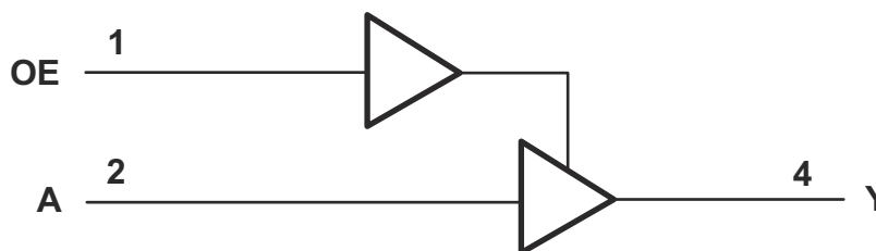
Figure 8-1. Logic Diagram
