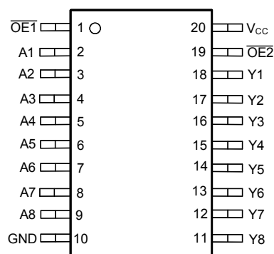
Figure 4-2. SN74LV8T541-Q1 PW, DGS Package (Top View)
