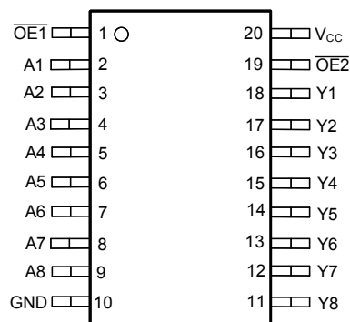
Figure 4-2. SN74LV8T9541-Q1 PW, DGS Package (Top View)
