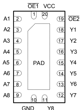
Figure 4-1. SN74LV8T9541-Q1 RKS Package (Top View)
